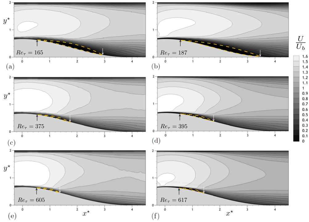
Figure 4: Contour plots of normalized streamwise velocity ( U/U_b ): (a) PIV at Re_\tau = 165 ; (b) DNS at Re_\tau = 187 ; (c) PIV at Re_\tau = 375 ; (d) DNS at Re_\tau = 395 ; (e) PIV at Re_\tau = 605 ; (f) DNS at Re_\tau = 617 . Black arrows denote the separation points and white arrows the reattachment points. Dashed lines denote the separation bubbles for all the cases presented.
