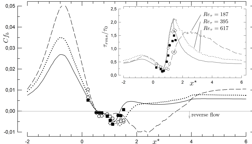
Figure 9: Skin friction coefficient over the bump surface plotted against x^* for three Reynolds-numbers (numerical and experimental dataset). Relative intensity of the wall shear-stress fluctuations are also plotted against x^* . \tau_0 denotes the mean wall shear stress evaluate at x^* = -6 . \circ Re_\tau = 165 , \diamond Re_\tau = 375 and \blacksquare Re_\tau = 605 . Lines represent numerical data (solid line; Re_\tau = 617 , short-dashed lines; Re_\tau = 395 and medium-dashed lines; Re_\tau = 187 ).
