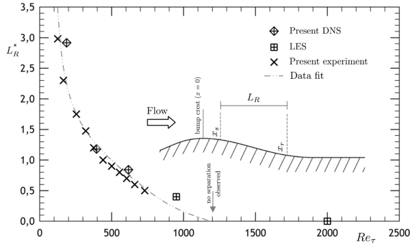
Figure 5: Normalized separation length, L_R^* , plotted against Re_\tau . Cross diamond symbols represent the present DNS data and cross square symbols represent the LES data from [41].
