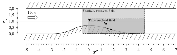
Figure 2: Test section containing the two-dimensional bump geometry and the PIV fields of interest. The symbol * denotes the half height normalization. \eta represents the direction of the local outward normal of the surface and \zeta the tangential direction.
