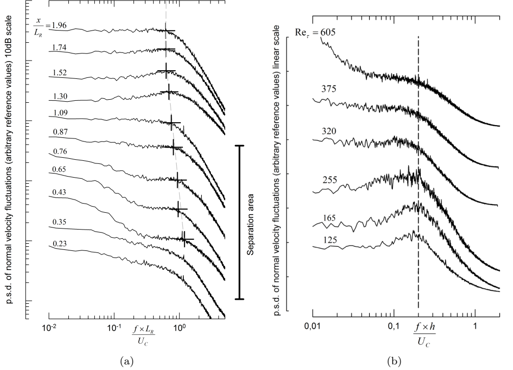
Figure 10: Power spectral densities (P.S.D) of the vertical fluctuating velocity component, v' , (a) at various x/L_R location along to the shear layer and at an elevation corresponding to the maximum of the velocity gradient locations for Re_\tau = 165 (b) at x/L_R \approx 1.5 for various Reynolds numbers. h/U_c is used in order to normalize the frequency and P.S.D are plotted with arbitrary reference scale.
