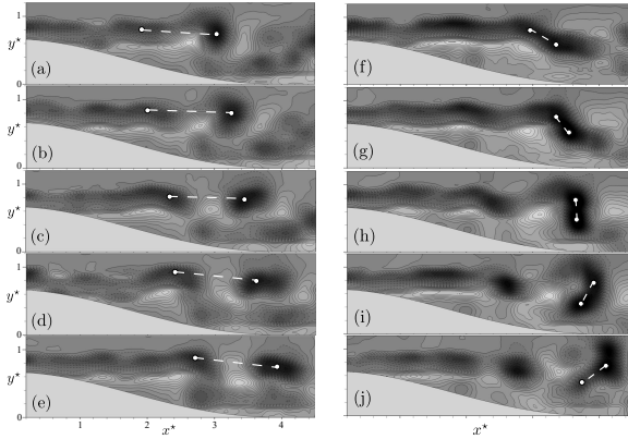
Figure 11: Two samples of the fluctuating vorticity field from the TR-PIV at Re_\tau = 125 showing different phases of the same shear layer vortex without (a to e) and with (f to j) self-interacting. Time steps follow from top to bottom and the normalized time interval between snapshot is \Delta t.U_b/h = 0.0216 . Arbitrary scale. \circ denotes dominant vorticity centers. The two vortices cores pointed out have a clockwise rotation.
