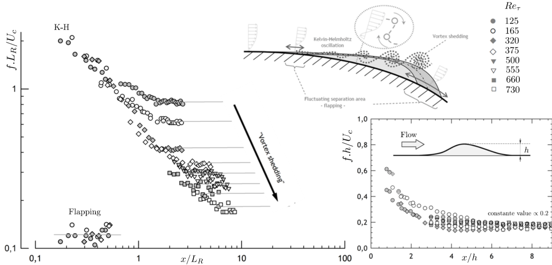
Figure 17: Normalized Frequencies peaks plotted against the distance from the separation location above the bump surface. The significant peaks are extracted from the wall-shear stress and from the velocity spectra. h denotes here the bump height.
