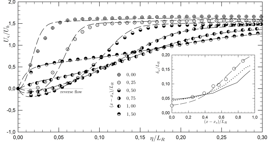
Figure 6: Normalized mean tangential component U_\xi at the channel symmetry plane ( z^* = 0 ) against \eta/L_R . The direction of the local outward normal of the surface for Re_\tau = 165/187 . The inset plot is the normalized vorticity thickness against (x - x_s)/L_R , x_s denotes the separation abscissa. \circ represent experimental data for Re_\tau = 165 . Lines represent numerical data (solid line; Re_\tau = 617 , short-dashed lines; Re_\tau = 395 and medium-dashed lines; Re_\tau = 187 ).
