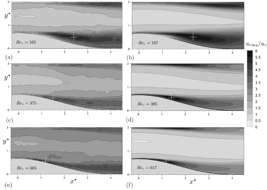
Figure 7: Contour plots of normalized streamwise r.m.s. velocity ( u_{rms}/u_\tau ): (a) PIV at Re_\tau = 165 ; (b) DNS at Re_\tau = 187 ; (c) PIV at Re_\tau = 375 ; (d) DNS at Re_\tau = 395 ; (e) PIV at Re_\tau = 605 ; (f) DNS at Re_\tau = 617 .
