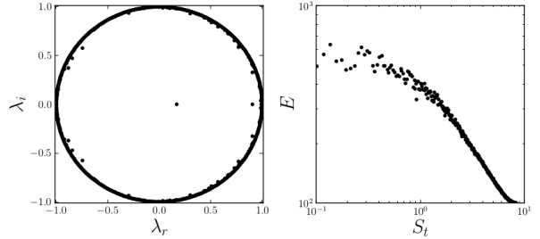
Figure 14: (Left): Spectrum of the Dynamic Mode Decomposition. (Right): The normalized kinetic energy norm versus the Strouhal number. Re_\tau = 617 .
