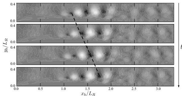
Figure 16: Evolution of the perpendicular component of velocity of the (K-H) mode for a Strouhal number St = 2 over one period T .
