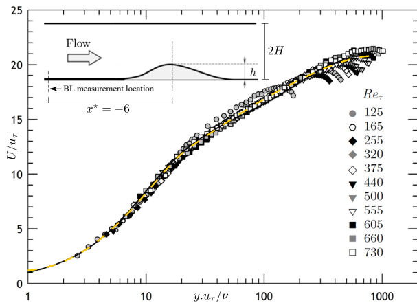
Figure 3: Profiles of the streamwise velocity against the wall-normal coordinate for various Reynolds-numbers. Dashed line represents DNS results of [26] at Re_\tau = 617
