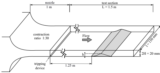
Figure 1: 3D view of the channel setup.
