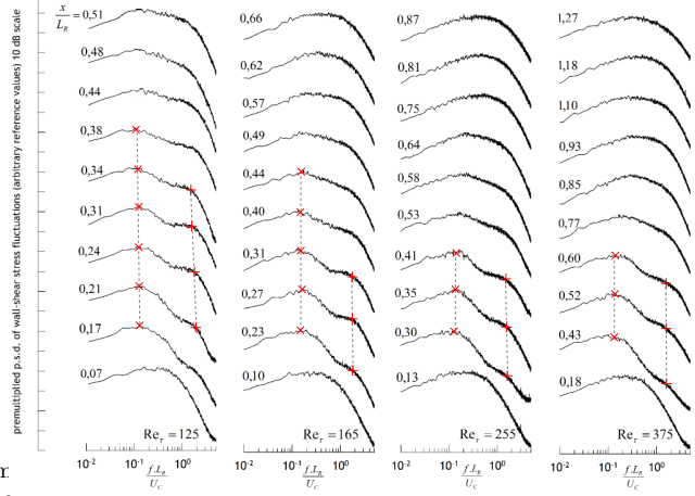
Figure 12: Weighted power spectrum density of the wall-shear stress fluctuations at various Reynolds-number against the distance x/L_R . + and x symbols denotes the spectrum peaks. The vertical dashed line shows the normalized low-frequency 0,12 and the inclined dashed lines denotes the evolution of the secondary spectrum peaks.
