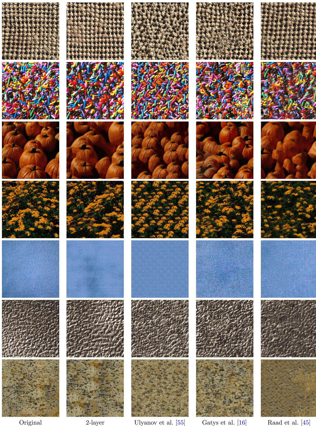
Fig. 11: Comparison. For each row, we display, from left to right, an original texture, the result of the model based on 2-layer patch transport, the result of the feed-forward network of [55], the result of the neural optimization procedure of [16] and the results of the patch-based method of [45]. See the text for comments.
