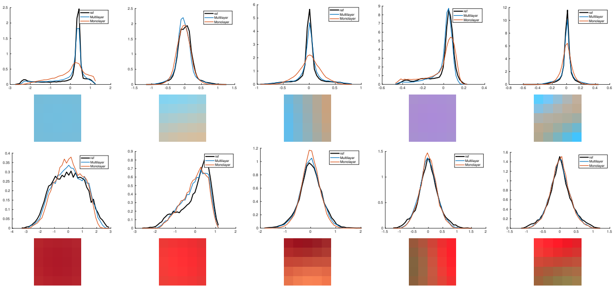
Fig. 8: Single-resolution model, output patch distributions. In this figure, we examine the output patch distributions after the mono-layer and bi-layer transport maps for the single-resolution model with patch size w = 5 , for the textures shown in the two first rows of Fig. 7. Each diagram represents the one-dimensional distribution obtained after projecting on a principal axis in the patch space, and the corresponding patch principal component is displayed just below. On each diagram, the black curve is the reference distribution, the blue curve is the distribution after multi-layer transport and the yellow curve is the distribution after mono-layer transport. See the text for comments.
