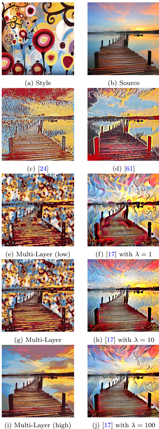
Fig. 20: Image stylization comparison of the proposed approach (20e, 20g and 20i) with other feed-forward techniques requiring learning over a dataset: Johnson et al. [24] (20c), Zhang et al. [61] (20d), or with pixel-wise optimization: Gatys et al. [17] (20f, 20h and 20j). See the text for comments.
