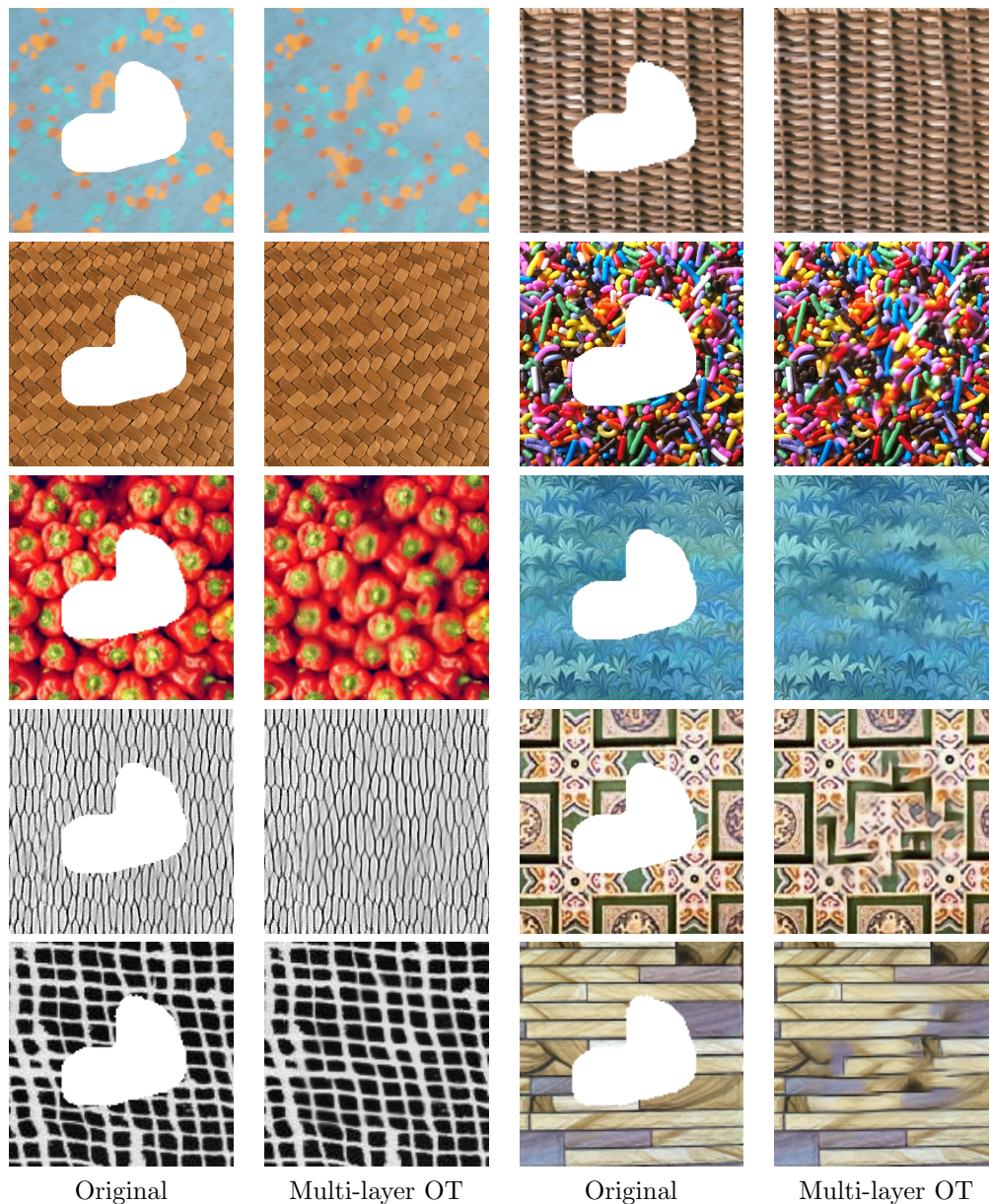
Fig. 15: Textural inpainting results. For several masked textures (1st and 3rd columns) we display the inpainting result obtained with the model based on 2-layer patch transport. Notice that the inpainted content blends quite nicely with the rest of the image, even if a residual blur is sometimes perceived due to patch averaging.
