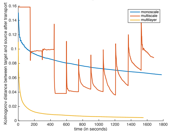
J = 10000 points
