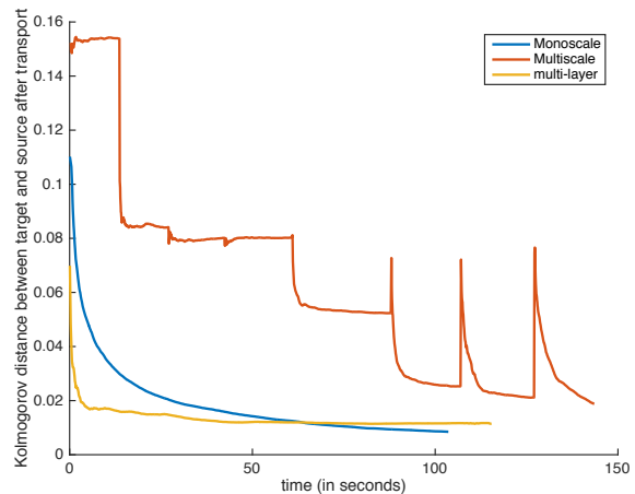
J = 1000 points
