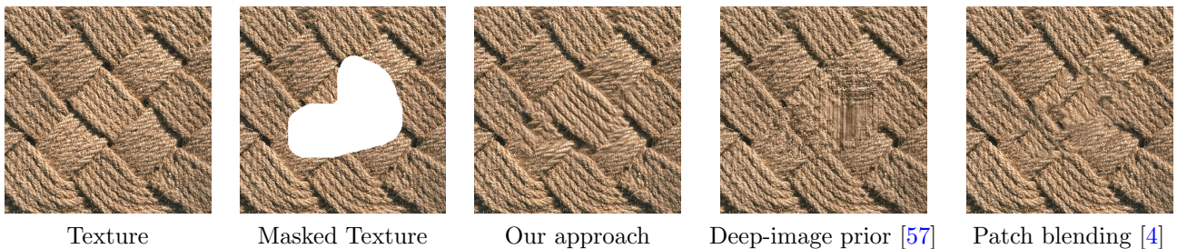
Fig. 17: Textural inpainting comparison. In this example we compare our approach with Deep image prior [57] (which optimizes a deep neural network with skipping connection to generate the masked image using Mean Square Error criterion) and with [4], where patches from the uncovered part of the image are used to fill in the masked domain and blended to avoid blocking artifacts.
