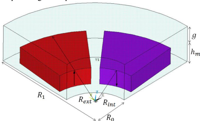
Fig. 1. A 3-D representation of a pair of poles of the AFPM machine.
