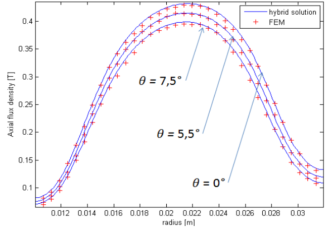
Fig. 4. Axial flux density as a function of the radial coordinate computed by hybrid analytical-FD method and FEM.
