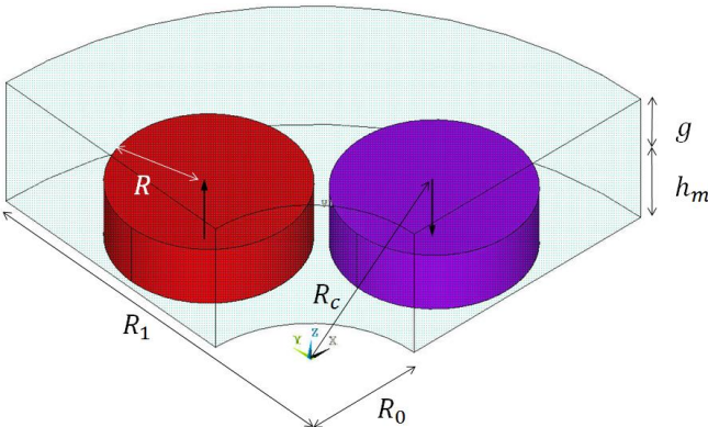
Fig. 3. 3-D view of the AFPM machine with circular shaped magnets.
