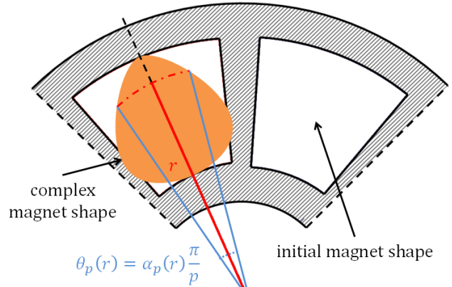
Fig. 2. Complex magnet shapes with arc pole depending on radial position.
