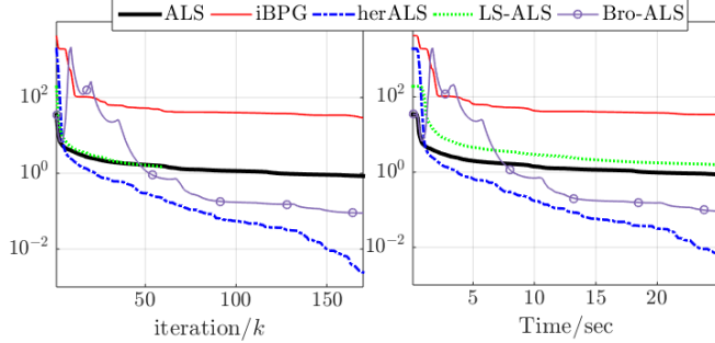
Fig. 2. Results on Wine [44, 2700, 200, 15]. iBPG gets stuck on local minima.
