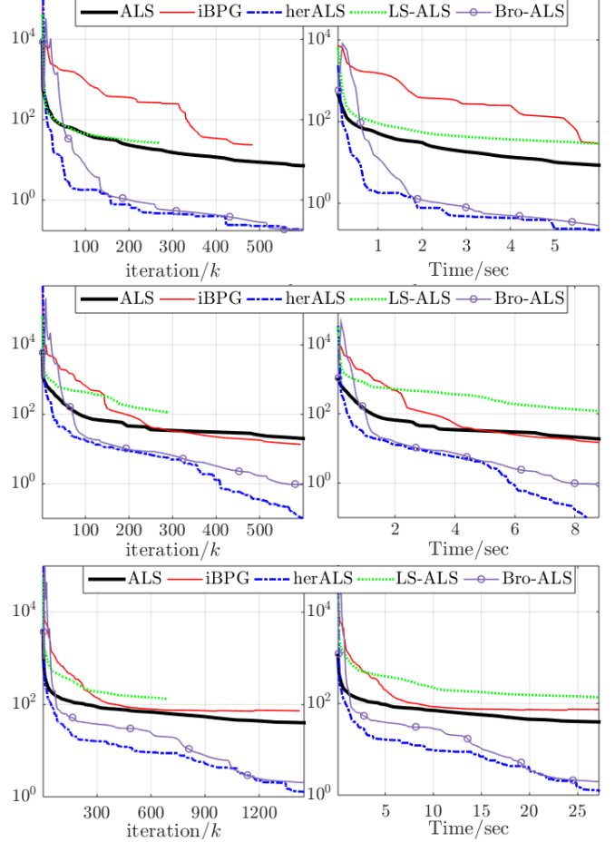
Fig. 4. Results on Blood [289, 301, 41] with r = 3 (top), r = 6 (mid) and r = 10 (bottom). Note that the data has many NaN (data polluted due to Rayleigh scattering), all NaN are replaced by 0. There are therefore many zero fibers in the tensor after such correction.
