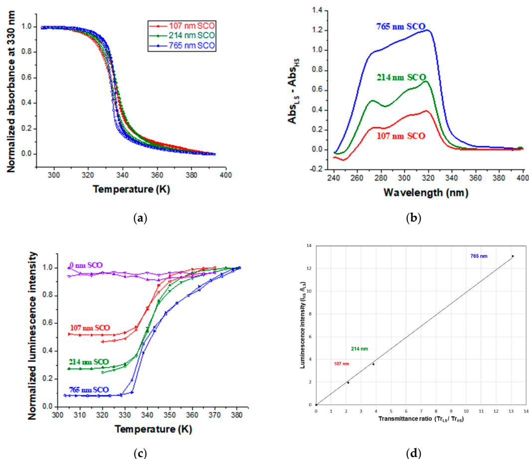
Figure 4. Correlation between the absorbance of [Fe(HB(tz)_3)_2] and the luminescence of Ir(PPy)_3 . (a) Normalized temperature dependence of the UV absorbance (at 330 nm) for three bilayer samples with different SCO layer thicknesses (107, 214 and 765 nm). (b) Absorbance changes associated with the SCO for different SCO film thickness. (c) Normalized temperature dependence of the luminescence intensity for different SCO film thickness. (d) Plot of the luminescence intensity ratio vs. the UV transmittance ratio between the HS and LS states. The corresponding SCO film thickness is also shown.
