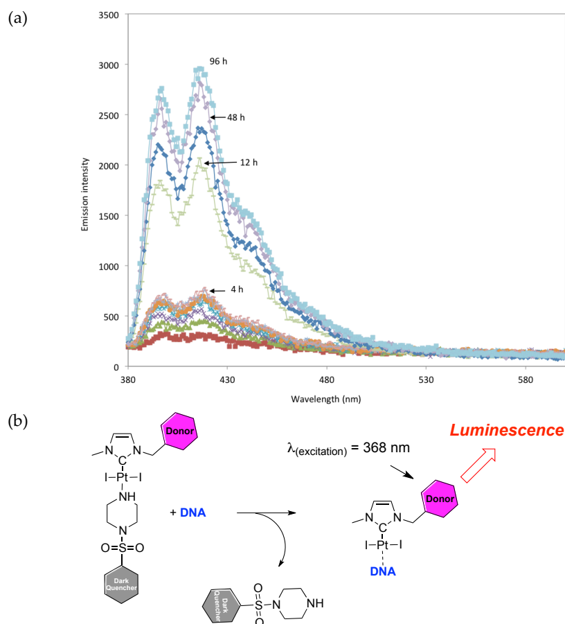
Figure 6. (a) Measurements of the emission spectra after excitation at \lambda = 368 nm (0.29 mg of 2 were dissolved in 50 \mu L of DMSO and added to a solution of 1.8 mg of salmon sperm DNA in water (1.950 mL), C_{Pt} = 1.34 \times 10^{-4} , (10 base pairs compared to Pt)). (b) Origin of the luminescence upon interaction with DNA ( 50 ).
