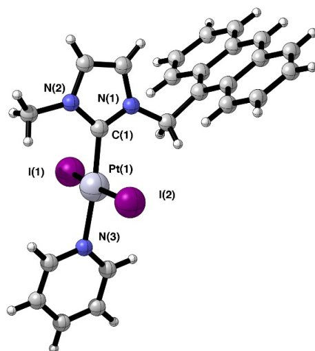
Figure 3. Molecular structure of the platinum complex 1 . Selected bond lengths ( \text{\AA} ) and angles ( ^\circ ): C(1)-Pt(1), 1.961(1); N(3)-Pt(1), 2.088(3); Pt(1)-I(1), 2.5732(3); Pt(1)-I(2), 2.6013(3); C(1)-Pt(1)-N(3), 174.88(14) ; C(1)-Pt(1)-I(1); 87.72(10) ; C(1)-Pt(1)-I(2), 92.03(10) ; I(1)-Pt(1)-I(2), 172.401(14) ; N(1)-C(1)-Pt(1)-I(1), -88.3(3) ; N(2)-C(1)-Pt(1)-I(1), 87.9(3) .
