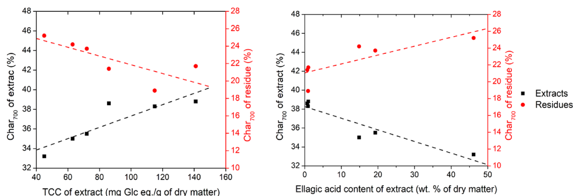
Figure 3. (A) Char yield at 700 °C of the chestnut wood extracts and residues versus total carbohydrate content (TCC) in the associated chestnut wood extracts. (B) Char yield at 700 °C of the chestnut wood extracts and residues versus ellagic acid content in the associated chestnut wood extracts. The standard deviations of triplicate assays are available in the Supporting Information .
