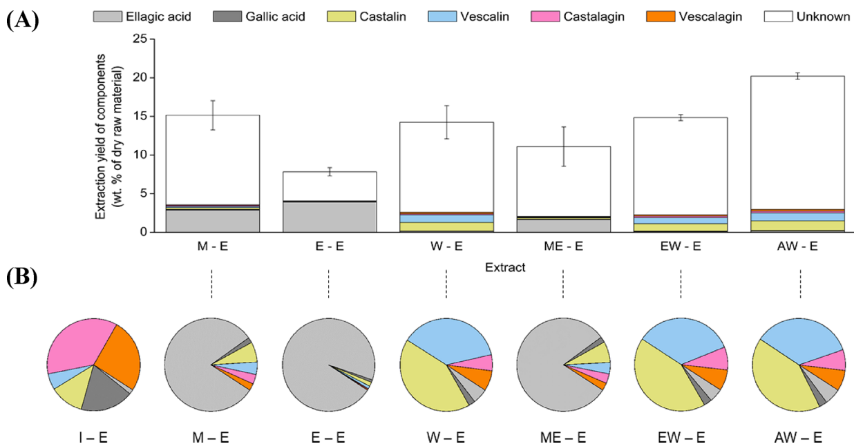
Figure 1. (A) Histograms are extraction yields (wt %) of extractives from ground chestnut sawdust, colored parts of which correspond to extraction yields of phenolic compounds. (B) Distribution of the six phenolic compounds (ellagic acid, gallic acid, castalin, vescalin, castalagin, and vescalagin) in the industrial (left) and lab-scale extracts.
