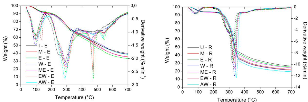
Figure 2. Thermograms of the chestnut wood extracts (left) and residues (right) at 10\text{ °C min}^{-1} under nitrogen flow as a function of solvent nature compared to the industrial extract (I-E) and the untreated chestnut wood (U-R).
