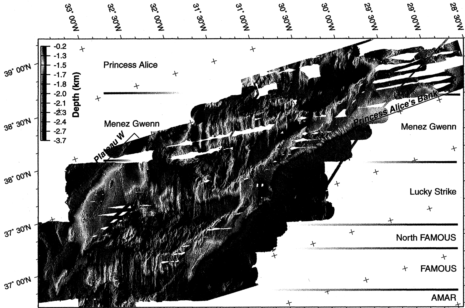
Plate 2. Oblique Mercator projection of high-resolution (~100-m grid spacing) shaded multibeam bathymetry of the study area (see Plate 1 and Figure 1). The horizontal grey/black bars indicate the approximate projection off axis of the present-day nontransform offsets bounding ridge segments. Note that the V ridges (Plate 1) are very shallow and present smooth topography, lack faults, and are covered with numerous seamounts (some >10 km in diameter). The seafloor within the V ridges show abyssal hill terrain subparallel to the ridge axis, typical of faulted slow-spreading oceanic crust. The shallowest portion of the V ridges off axis from the North FAMOUS and Lucky Strike segments are referred to as the west and east Jussieu Plateau, and the shallow zone of the east branch of the V ridge at ~29°N corresponds to Princess Alice Bank; no data from the conjugate side are available.
