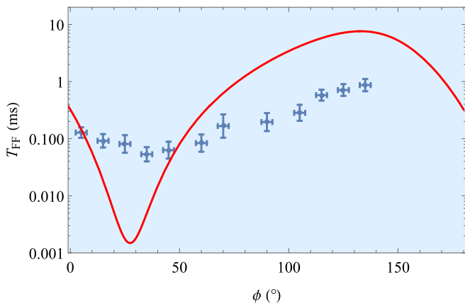
FIG. 5. Variation of the spin lifetime (log scale) with the angle \phi of an external magnetic field of 0.15 mT in the D_1 - D_2 plane for the 50-ppm crystal. The experimental measurements correspond to the optical inversion recovery technique only.
