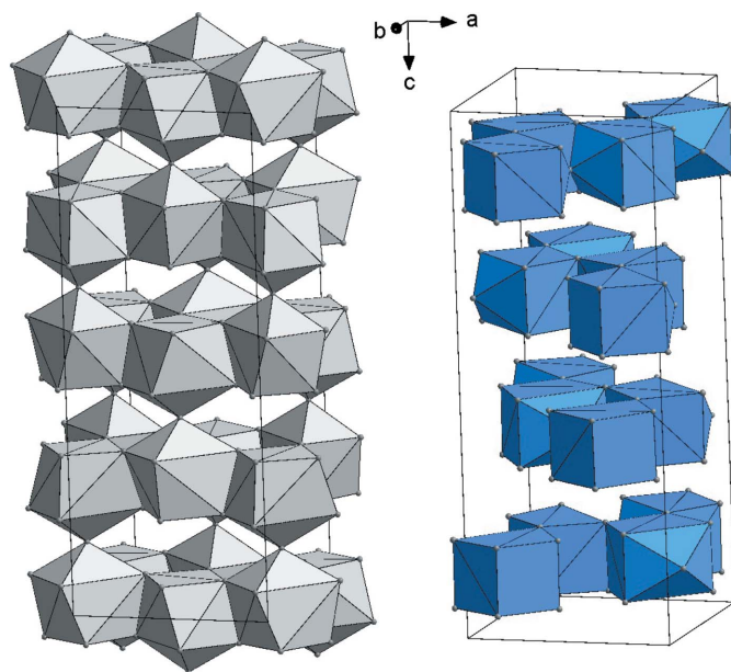
Figure 4 Distribution of the Al polyhedra built around the Au1/Ir1 (left) and Au2/Ir2 (right) atomic positions in the unit cell of the \text{Al}_9(\text{Au};\text{Ir})_4 compound reported here. Au1/Ir1 polyhedra are connected by sharing Al3 positions along the c axis and Al1–Al1 or Al2–Al2 edges in the (ab) plane. Au2/Ir2 polyhedra are only connected in the (ab) plane by sharing Al3 positions or Al1–Al2 edges.
