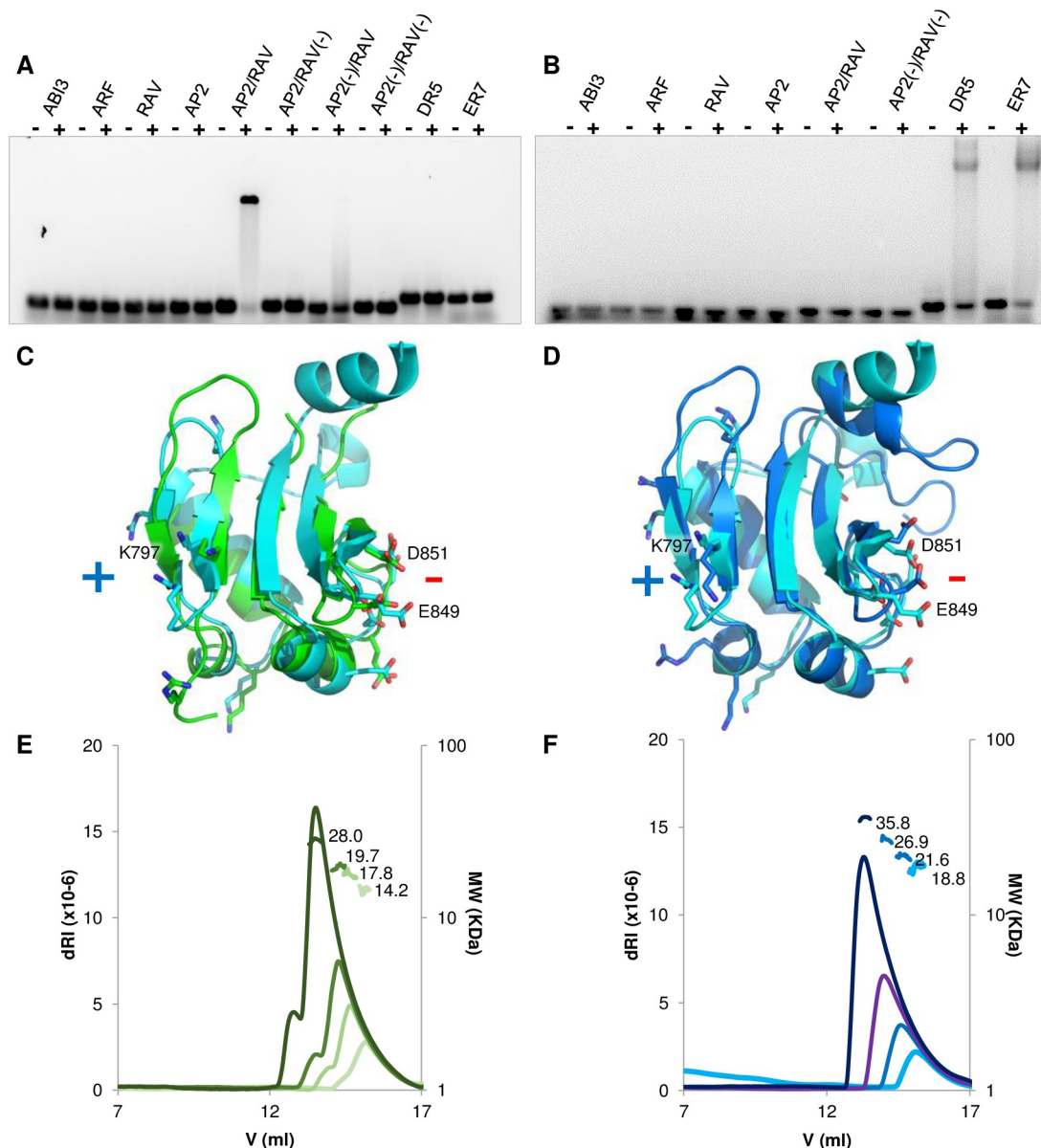
Fig 2. Proto-RAV and proto-ARF biochemical properties. (A), KNRV-DBD (AP2/B3 domains) or (B), Ca-ARF-DBD interactions in EMSA with specific single binding sites for different B3 families (ABI3, ARF and RAV) [45], AP2, a composite site for AP2-B3/RAV family, AP2(-)/RAV mutated on AP2, AP2/RAV(-) mutated on RAV, AP2(-)/RAV(-) mutated on both AP2 and RAV, DR5 (Direct Repeats AuxRE spaced by 5 nucleotides) and ER7 (Everted Repeats spaced by 7 nucleotides) ARF motifs. DNA sequences are indicated in S8 Table. Proteins added at 0 and 0.5 \mu M. (C-D), Structure models for KNRV-PB1 (C, green) and CaARF-PB1 (D, blue) superposed to AtARF5-PB1 structure (cyan) (PDB code 4CHK [23]). Conserved residues indicated refer to AtARF5-PB1 structure. Positive and negative signs indicate potential interaction surfaces for oligomerization. (E), SEC-MALLS KNRV-PB1 molecular weight determination for four protein concentrations (from dark to light green: 5 mg/mL, 2.5 mg/mL, 1.25 mg/mL and 0.625 mg/mL). (F), SEC-MALLS CaARF-PB1 molecular weight determination (from dark to light blue: 5 mg/mL, 2.5 mg/mL, 1.25 mg/mL and 0.625 mg/mL).
