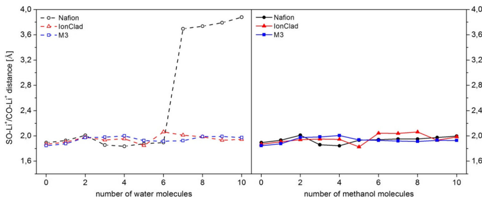
Fig. 3 Minimal distance between sulfonyl group and \text{Li}^+ counterion in Nafion, IonClad, and M3 membranes vs. number of absorbed water (left) and methanol molecules (right)
