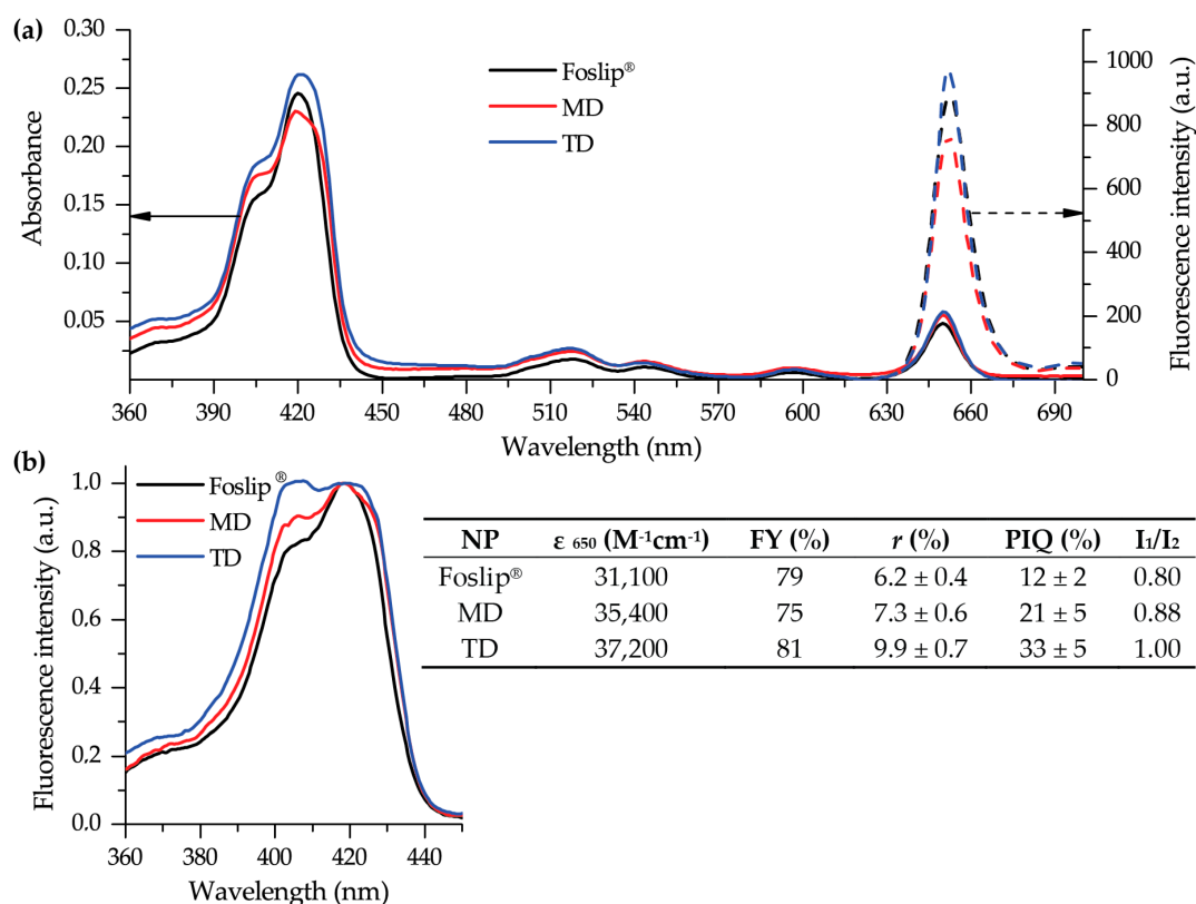
Figure 3. Spectral characteristics of Foslip ® (black), MD (red), and TD (blue) in PBS. (a) Absorbance (solid line) and fluorescence emission (dotted line) spectra ( \lambda_{ex} = 420 nm); (b) normalized fluorescence excitation spectra ( \lambda_{em} = 652 nm). mTHPC concentration was 1.5 \mu M . Insert shows the main spectral characteristics of NPs, such as extinction coefficient at 650 nm ( \epsilon_{650} ); FY—fluorescence yield, relative to the fluorescence of mTHPC in ethanol; r —the degree of fluorescence anisotropy; PIQ—the degree of photoinduced quenching; I_1/I_2 —the ratio of Soret band components ( I_1 and I_2 were measured under excitation at 407 nm and 418 nm, respectively, and emission at 652 nm).
