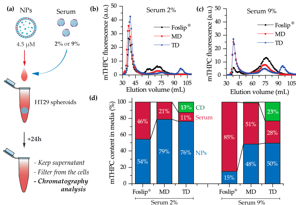
Figure 7. (a) Scheme of the experiment; (b,c) chromatography histograms of culture medium after 24 h incubation of HT29 spheroids with mTHPC (4.5 \mu M) in nanoformulations in the presence of (b) 2% and (c) 9% of serum; (d) the percentage of mTHPC bound with NPs (blue) or serum proteins (red) and in complexes with CDs (green).
