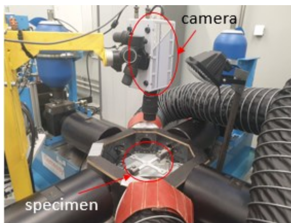
Figure 4. Biaxial testing machine
