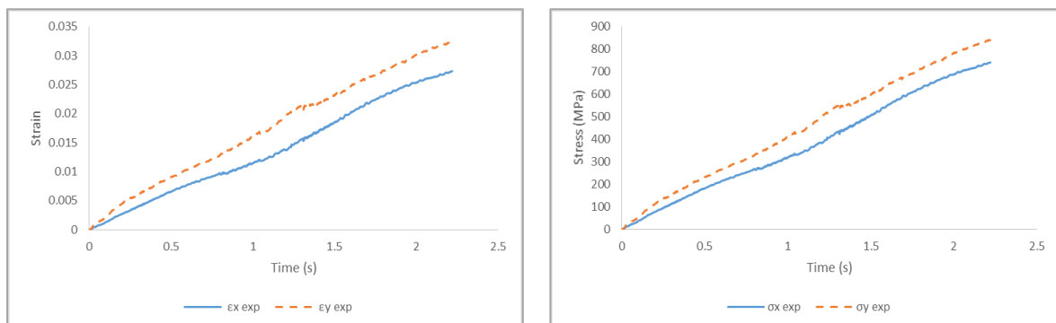
Figure 12. Strain (left) and stress (right) in the central zone for Test03
