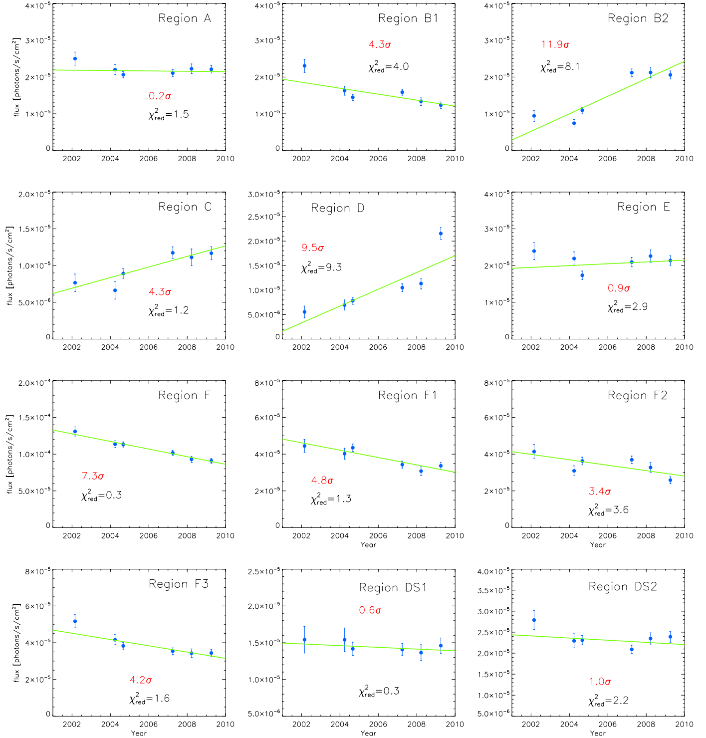
Fig. 4. Lightcurves of the Fe-K \alpha flux from the filaments in the GC. The flux is plotted in units of 10^{-5} photons \text{cm}^{-2} \text{s}^{-1} . The green line represents the best fit linear function to the data, whose parameters are reported in Table 4. In each panel we present the significance of the measured gradient ( B/\sigma_B ) together with the \chi^2_{\text{red}} for the best fit linear function.
