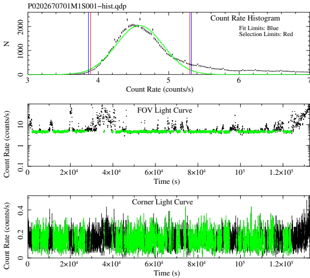
Fig. 1. Soft proton flare filtering of the MOS1 dataset from OBSID 0202670701. Upper panel: 2.5–12 keV count rate histogram. The blue lines mark the region used in the Gaussian fit, the green line represents the best fit Gaussian and the red lines show the bounds used to filter the data. Mid panel: 2.5–8.5 keV lightcurve of the IN FOV region. Lower panel: 2.5–8.5 keV lightcurve of the corner data. In both the Mid and the Lower panels, the points coloured green in the light-curves correspond to the selected GTI intervals (see text).
