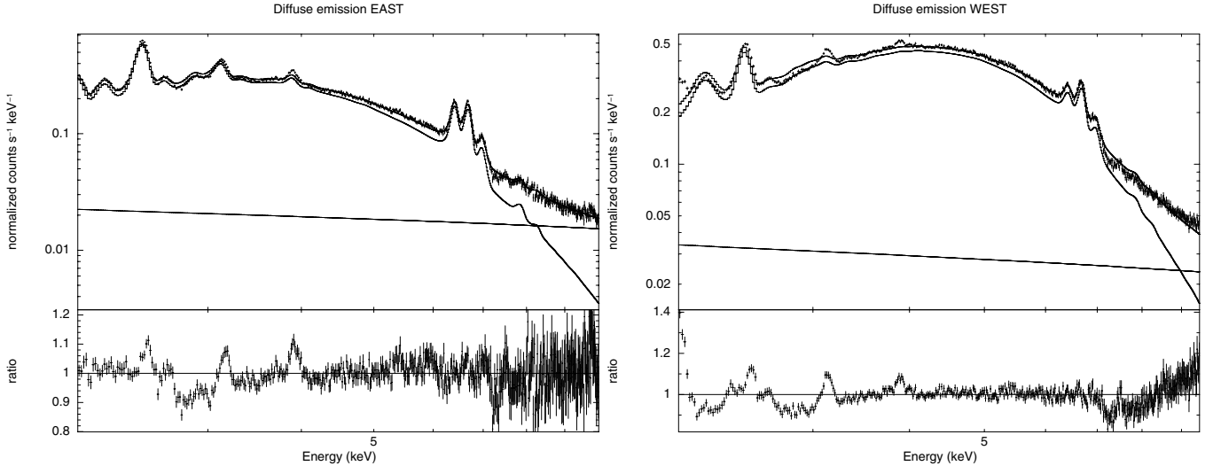
Fig. 12. Left panel: MOS2 spectrum of the EDE region, with the residuals in the bottom panel. The data have been collected stacking all the MOS2 spectra of the region from all the observations. Right panel: same for the EDW region.
