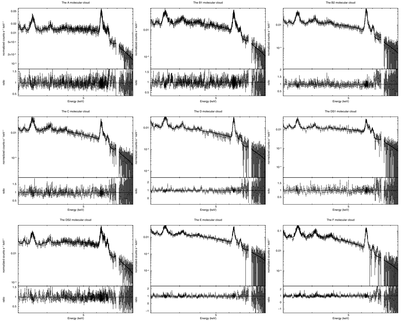
Fig. 6. Time-averaged PN spectra of the set of MCs in the present study. Each panel shows the measured data along with the best fitting spectral model and (in the lower section) the ratio of these two quantities. The spectral channels encompassing the Cu-K \alpha line at 8.05 keV (7.8–8.2 keV) have been excluded from the fitting.
