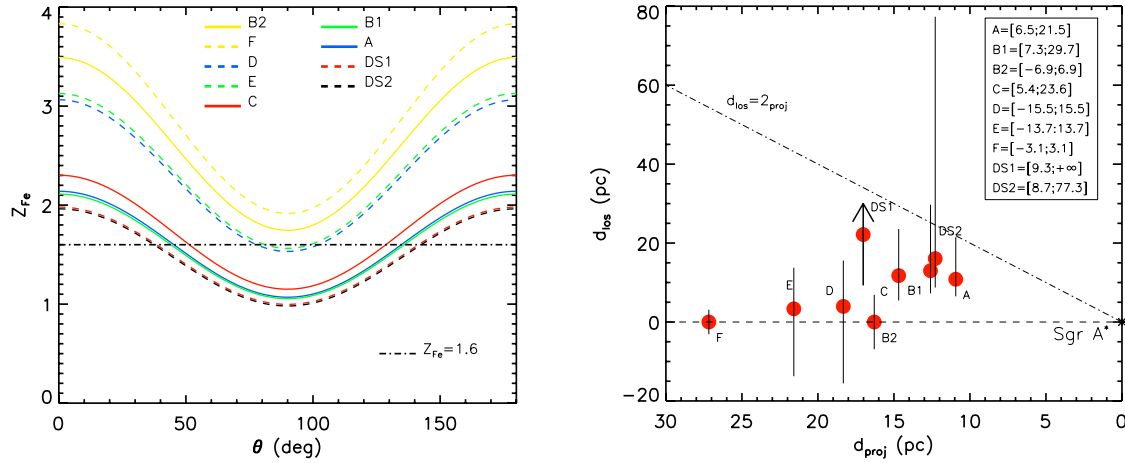
Fig. 8. Left panel: relative Fe abundance Z_{\text{Fe}} as a function of the scattering angle \theta for the different MCs obtained by using the measured EW and Eq. (3). The horizontal dashed-dotted line represents the average metallicity ( Z_{\text{Fe}} = 1.6 ) inferred for set of MCs. Right panel: line-of-sight displacement plotted against the projected distance d_{\text{proj}} for each MC. The d_{\text{los}} value for the DS1 cloud is a lower limit ( d_{\text{los}} \geq 9.3 pc). The horizontal dashed line represents the plane of Sgr A* at d_{\text{los}} = 0 . The dashed-dotted line shows the line d_{\text{proj}} = 2 \times d_{\text{los}} . We make the assumption that the clouds are located in the region between the dashed and dashed-dotted lines (see text). The permitted d_{\text{los}} range (in pc) for each cloud is given in the top-right box. Note: the method does not distinguish between whether an individual cloud lies in front or behind the plane of Sgr A* (i.e., at +ve or -ve d_{\text{los}} ).
