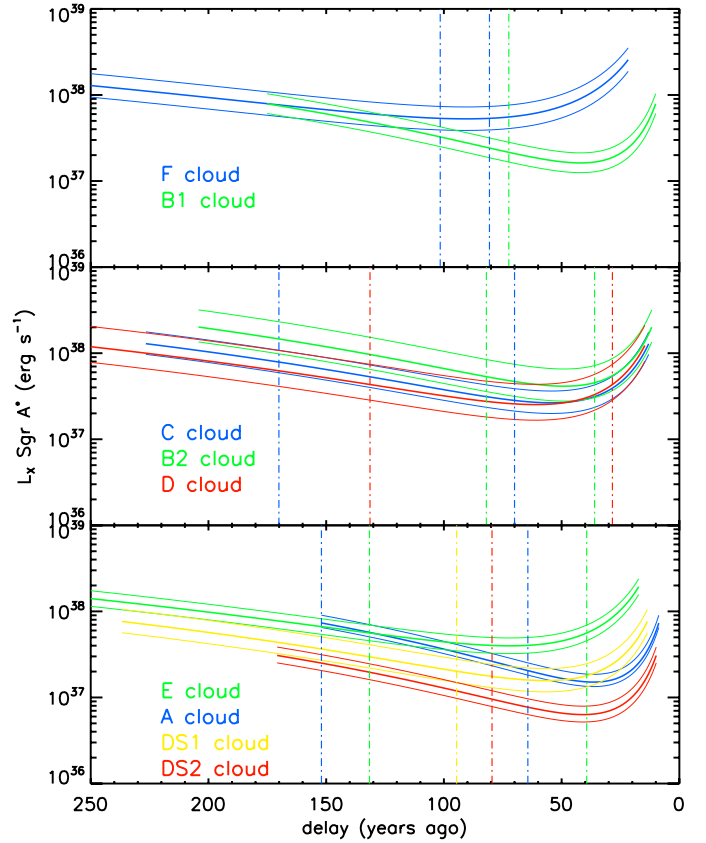
Fig. 9. X-ray luminosity as a function of the time delay for the different MCs, as inferred from the measured cloud properties. We have divided the MCs into subgroups depending on the type of Fe-K \alpha line variability exhibited. Also plotted are the 90% confidence ranges on the L_X calculation. The vertical dotted lines represent the constraints on \theta derived in Sect. 4.1. Where only one vertical line is shown for a cloud, it represents the right-hand boundary of the allowed range; in these cases the second boundary is situated to the left of the Y axis (i.e., \theta \geq 155 deg), and therefore not plotted.
