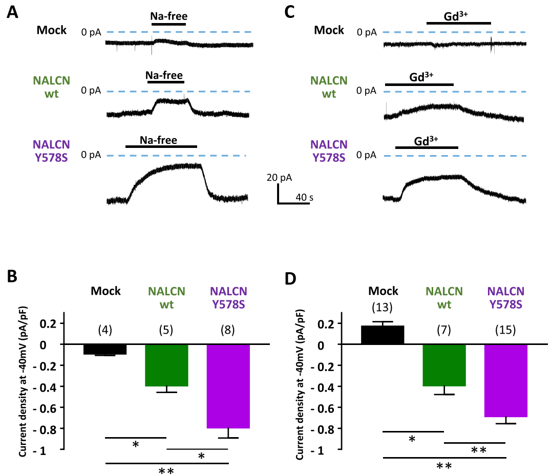
Figure 2. Transient expression of the wild-type (wt) NALCN and its CLIFAHDD variant Y578S together with NLF1 in differentiated NG108-15 cells results in the expression of a NMDG- and Gd^{3+} -sensitive background Na^+ current. (A) Representative traces obtained on cells held at -40 mV (HP) during application/wash of an extracellular Na^+ -free solution (replaced with NMDG) for a mock (NLF1)-transfected cell (top), a NALCN/NLF1 (wt)-transfected cell (middle), a NALCN CLIFAHDD mutant (Y578S)/NLF1-transfected cell (bottom). (B) Density of the external Na^+ -dependent background current ( Na^+ -free) for mock-transfected cells ( -0.088 \pm 0.03 pA/pF, n = 4 ); NALCN: -0.391 \pm 0.14 pA/pF, n = 5 ; NALCN-Y578S: -0.79 \pm 0.32 pA/pF, n = 8 ). (C) Representative traces obtained on cells held at -40 mV during application/wash of Gd^{3+} ( 10 \mu M ) for a mock-transfected cell (top), a NALCN (wt)-transfected cell (middle), a NALCN CLIFAHDD mutant (Y578S)-transfected cell (bottom). (D) Average density of the Gd^{3+} -sensitive background current for mock-transfected cells ( 0.168 \pm 0.16 pA/pF, n = 13 ), NALCN (wt)-transfected cells ( -0.391 \pm 0.23 pA/pF, n = 7 ) and NALCN-Y578S-transfected cells ( -0.684 \pm 0.27 pA/pF, n = 15 ). Both the Na^+ -dependent background current and the Gd^{3+} -sensitive background current were significantly of higher density for wt NALCN and its pathogenic variant Y578S compared to the control condition ( p = 0.03 and 0.004 for the Na^+ -dependent component and P < 0.0001 and < 0.0001 for the Gd^{3+} -sensitive component respectively). In addition, densities of the Na^+ -dependent background current and the Gd^{3+} -sensitive background current were significantly lower for wt NALCN compared to its pathogenic variant Y578S ( p = 0.045 and p = 0.029 respectively). p values were calculated with a Mann-Whitney statistical test.
