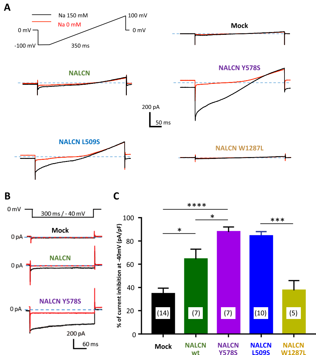
Figure 3. Amplitude of the Na + -dependent component of the NALCN current carried out by the CLIFAHDD variants (Y578S, L509S) and the IHPRF variant (W1287L) of the NALCN channel. (A) Representative current traces elicited by a voltage ramp protocol (from -100 mV to +100 mV) in the presence (black traces) and in the absence (red traces) of extracellular Na + . (B) Representative current traces elicited by a voltage step protocol (HP 0 mV, test pulse (TP) at -40 mV) in the presence (black traces) and in the absence (red traces) of extracellular Na + . (C) Percentage of current inhibition obtained in Na + -free condition, for mock-transfected cells (34.51 ± 18.37%, n = 14), for NALCN-transfected cells (64.41 ± 22.67%, n = 7), for NALCN-Y578S-transfected cells (87.81 ± 11.2%, n = 7), NALCN-L509S-transfected cells (84.25 ± 12.06%, n = 10) and for NALCN-W1287L-transfected cells (37.56 ± 12.06%, n = 5). Compared to the control condition, the percentage of inhibition was significantly larger for NALCN-wt (p = 0.026), NALCN-Y578S (p < 0.0001), NALCN-L509S (p < 0.0001) but not for NALCN-W1287L (p = 0.864). A significant difference in the percentage of inhibition was also found for NALCN-wt compared to its pathogenic variant Y578S (p = 0.017) but not for L509S (p = 0.157) and W1287L (p = 0.197). P values were calculated with a Mann-Whitney statistical test.
