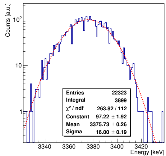
Close-up Proton Energy Peak (LOWER PLATE)
