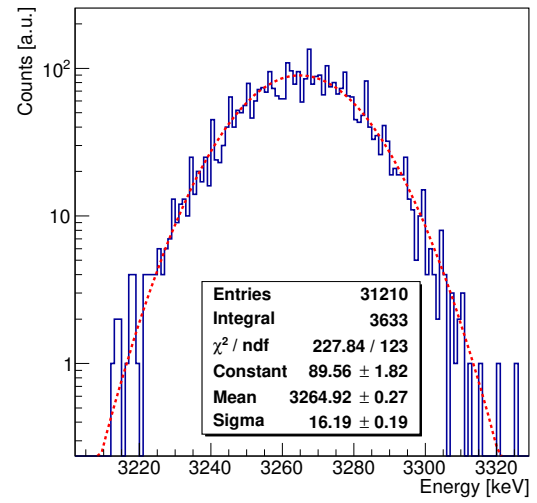
Close-up Proton Energy Peak (UPPER PLATE)
