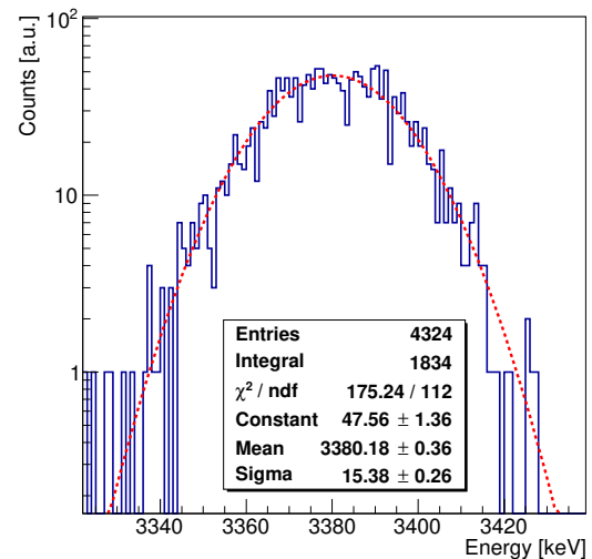
Close-up p-beta coincidence (LOWER PLATE)
