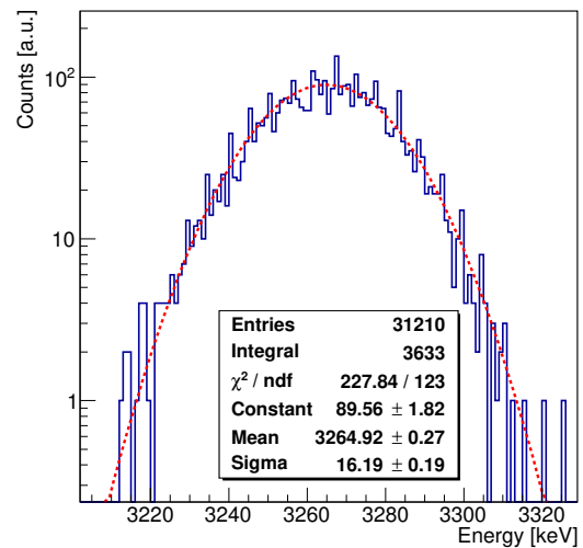
Close-up Proton Energy Peak (UPPER PLATE)
