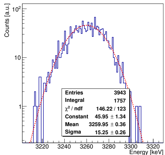
Close-up p-beta coincidence (UPPER PLATE)
