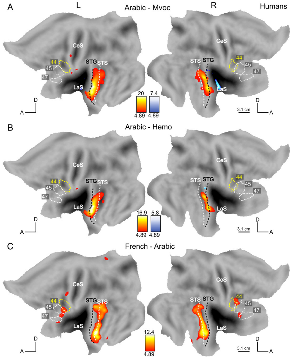
Figure 9: Processing of speech and intelligibility in humans. SPM T-map ( p < b 0.05 FWE corrected) for contrast Arabic-Mvoc (A), Arabic-Hemo (B) and French-Arabic (C) masked exclusively with effect of scrambling ( p < b 0.05 uncorrected) and shown in a red (positive)-blue (negative) color map.
