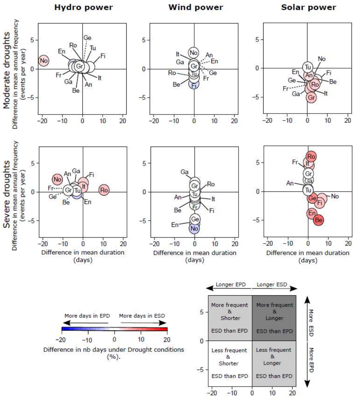
350 351 Fig.6: Difference in statistical characteristics from Energy Supply Droughts to Energy 352 production Droughts (ESD-EPD). x-axis: difference in mean duration of drought sequences; y-axis: 353 difference in annual frequency. Colour scale: difference in the number of days in drought state over the 354 simulation period.
