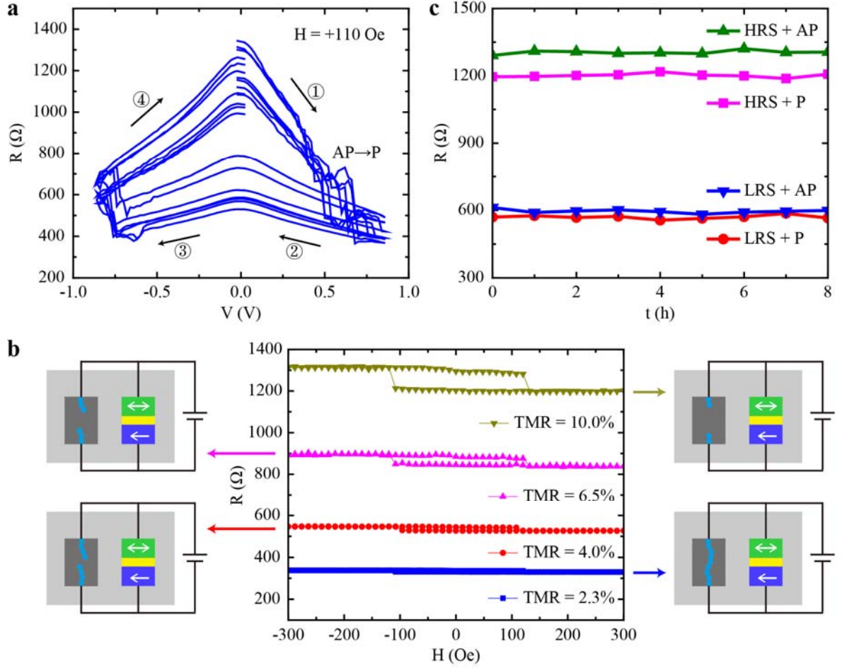
Figure 5. Multilevel resistance states in the Re-MTJ device. (a) Seven different R-V curves under external magnetic fields in the same device. (b) R-H hysteresis loops with different initial resistance states for the same device. The measurements were conducted from an LRS (approximately 600 \Omega ) to an HRS (approximately 1300 \Omega ). (c) Time-independent resistance curves showing the non-volatile features of the Re-MTJ for four different resistance states (LRS+AP, LRS+P, HRS+AP and HRS+P).
