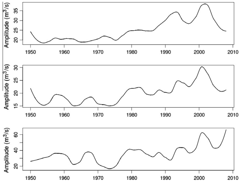
Fig. 8. Temporal distribution of amplitudes for the first three components of daily Seine river flow. Amplitudes increase significantly since the mid-1970s and seem modulated by an interannual scale of variability, leading to a pseudo-periodicity of the short-term amplitudes.
