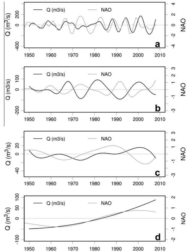
Fig. 11. Comparison between daily flow and winter-months NAO interannual components obtained from EEMD. The lower panel represents the Seine river flow EEMD residue (black line) and the ~77-years long-term component of NAO.
