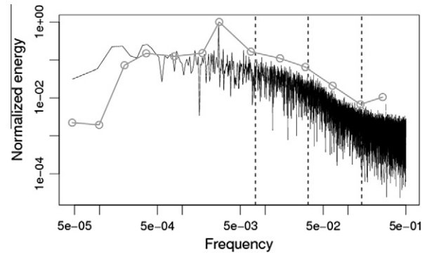
Fig. 4. Fourier energy spectrum (black solid line) and Hilbert Spectrum based on EEMD of daily Seine river flow. Dotted vertical lines indicate the detected range of scale invariance.
