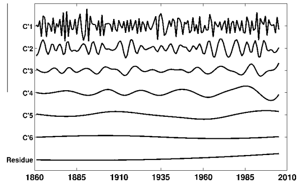
Fig. 9. EEMD of the winter-months annual NAO index time series from 1865 to 2008.
