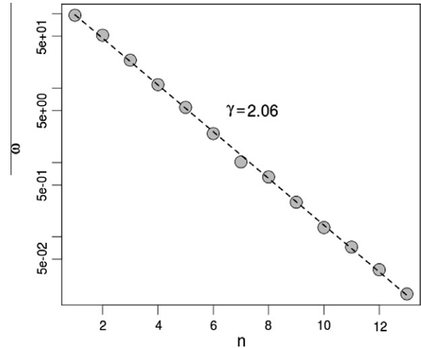
Fig. 3. Decreasing frequency with increasing order of the IMFs. The evolution of mean frequency with IMFs obeys a power law of the form \omega(n)=\gamma - n with \gamma = 2.06 , showing that the EEMD algorithm acts as a dyadic filter bank.
