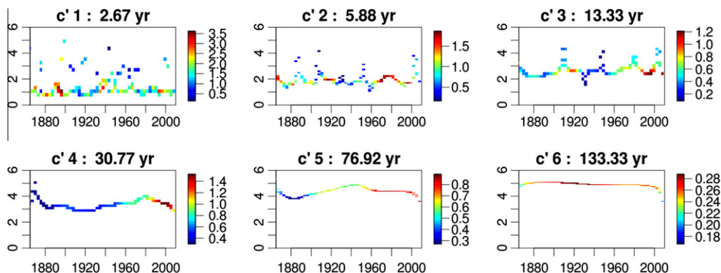
Fig. 10. Instantaneous frequency trajectories from Hilbert–Huang Transform (HHT) applied to each component (IMF) of winter-months NAO extracted from EEMD. The color scale indicates normalized unit of the NAO index.
