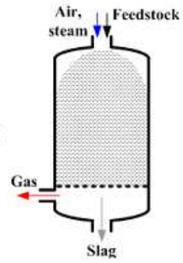
Entrained flow gasifier
