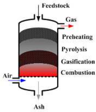
Moving bed gasifier
