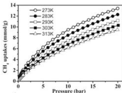
Figure 9. CH 4 adsorption isotherms on starch chars (CO 2 -activated at different temperatures)
