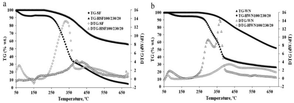
Figure 3. TG and DTG curves of precursors and respective hydrochars for a) sunflower stem and b) walnut shells under different hydrothermal conditions (Reproduced with permission from [63]).
