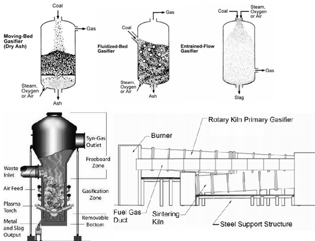
Figure 6. Types of char gasifiers (adapted from [146] and [147])
