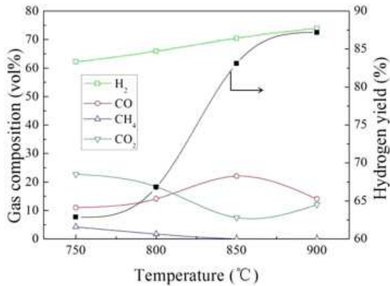
Figure 8. Effect of temperature on hydrogen yield from wheat straw char gasification
