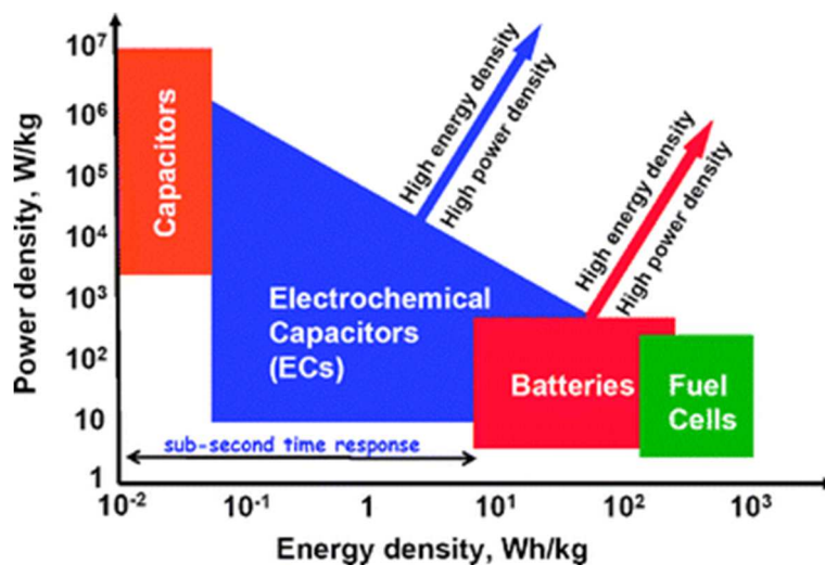
Figure 10. Common energy storage devices [193] (Reproduced by permission of The Royal Society of Chemistry)
