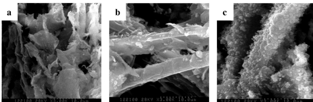
Figure 7. SEM images of char after the experiment at 700 °C under microwave heating. (a) Fresh char; (b) char from toluene reforming; (c) char from toluene cracking) (Reproduced with permission from [159]).
