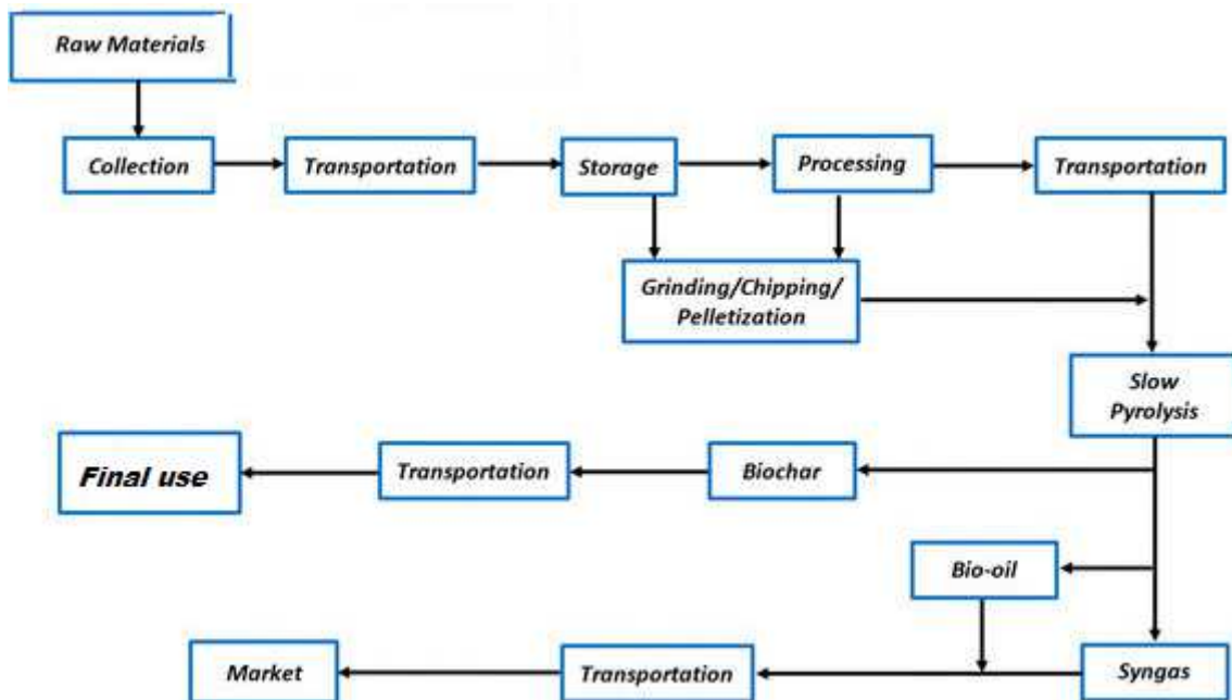
Figure 1. Industrial biochar system (Adapted from [24])
