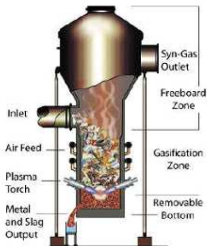
Plasma gasifier
