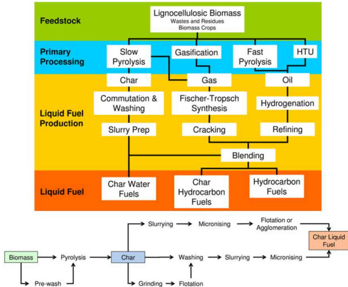
Figure 4. Pathways from biomass-derived chars to liquid fuels (Reproduced with permission from [133])
