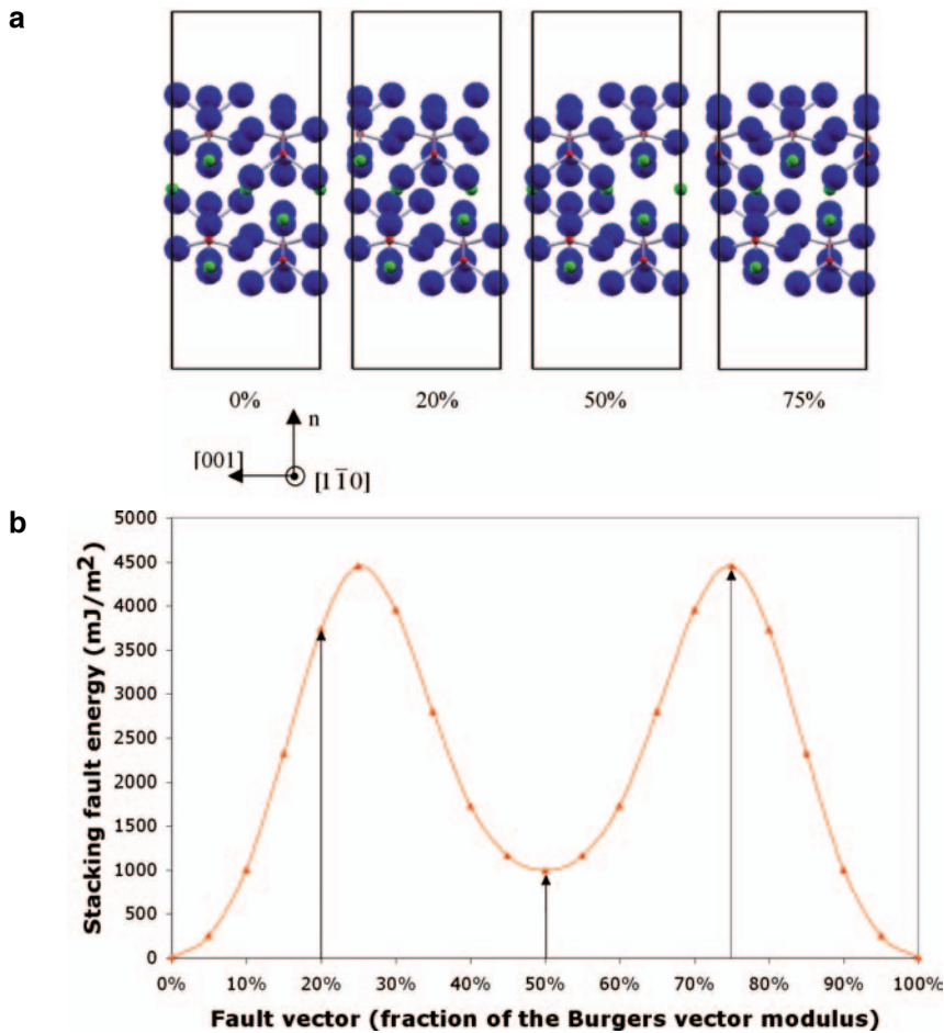
Fig. 3. Generalised stacking faults. (a) Supercell used to investigate plastic glide resistance in forsterite along [001] on (110). The unsheared supercell is presented on the left whereas three shear stages (20%, 50 % and 75% of the [001] lattice vector) are presented on the right side. (b) Energy barrier associated with [001](110) plastic shear.
