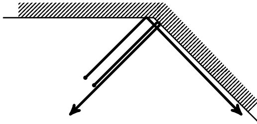
Figure 1. Non-continuous dependence of the solution on the initial datum.
