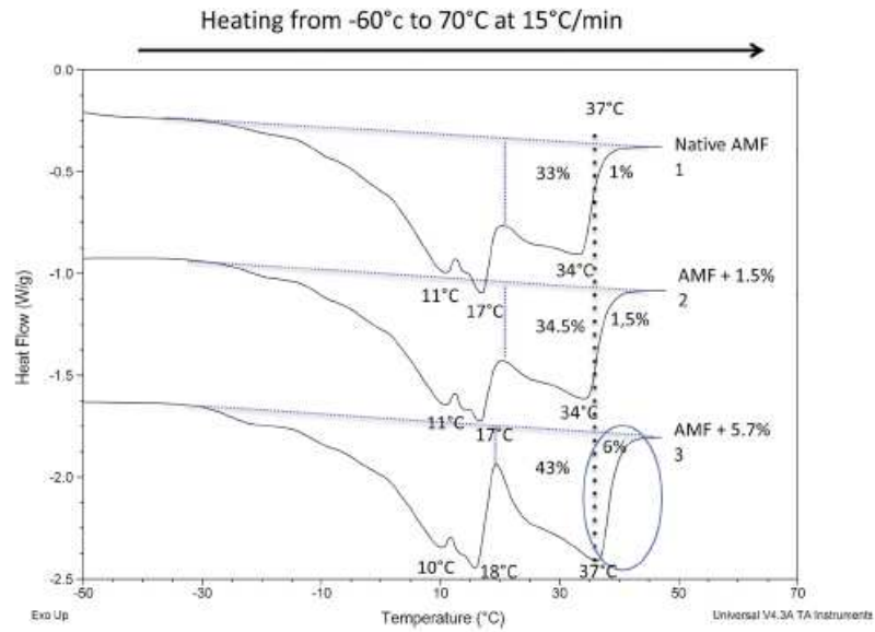
Figure 4. DSC melting profiles ( A =cooling curves recorded at -10^{\circ}\text{C}/\text{min} , B =heating curves recorded at 15^{\circ}\text{C}/\text{min} ) of native AMF (curve 1), AMF containing 1.5% external TAGs as tracers (curve 2), AMF containing 5.7% external TAGs as tracers (curve 3). NB: The tracer TAG mixture was composed of PPP, OOO and CCC in a 3 : 2.1 : 0.9 ratio.
