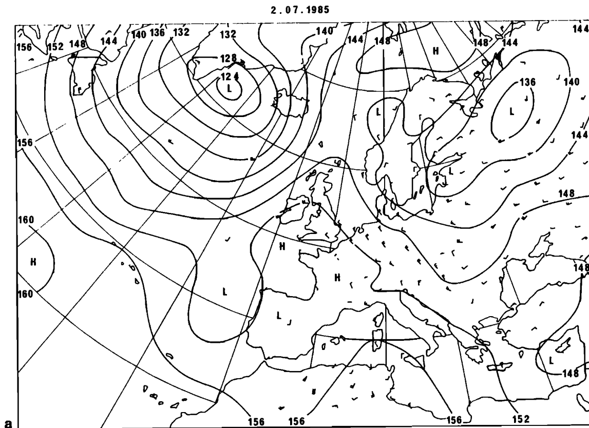
Fig. 1. Synoptic meteorological situation at 850 hPa around the Mediterranean area on (a) July 2, (b) July 3, and (c) July 4, 1985.
