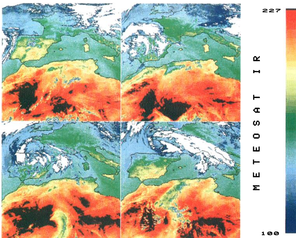
Plate 2. Colored Meteosat IR images (July 1 to 4, 1985, slot 24) showing the dusts over Africa (in green). The dust source region is visible in northern Algeria on July 1 and 2. A dust plume coming from the south is visible on July 3 and 4. The color table is linearly distributed between the numeric counts 100 (-6.5°C) and 227 (51°C). Pixels with their counts in the outer range are thresholded in white (cold) and black (warm). (Photo European Space Agency and Centre des Faibles Radioactivités).
