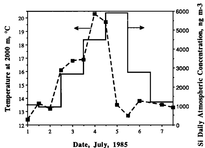
Fig. 5. Daily (noon to noon) mean atmospheric particulate concentration of Si at Capo Cavallo and air temperature at the altitude of 2000 m as deduced from available rawind soundings from July 1, 0000 UT, to July 7, 1200 UT. The July 6, 1200 UT, sounding is missing.
