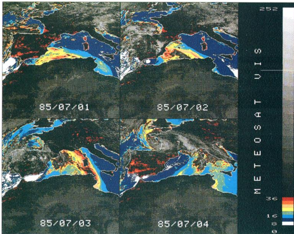
Plate 1. Colored Meteosat VIS images (July 1 to 4, 1985, slot 24) showing the transport of a dust plume over the western Mediterranean basin. Pixels with their numeric count at 8 (the lowest value in these images) are displayed in white, pixels at 12 in dark blue, pixels at 16 in light blue, ..., pixels at 36 in red. Pixels with upper values are black and white shaded. (Photo European Space Agency and Centre des Faibles Radioactivités).
