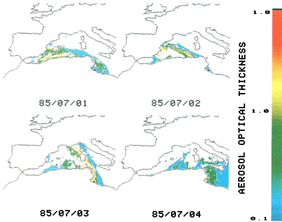
Plate 3. Calculated aerosol optical thickness over the western Mediterranean at 1145 UT from July 1 to 4, 1985.
