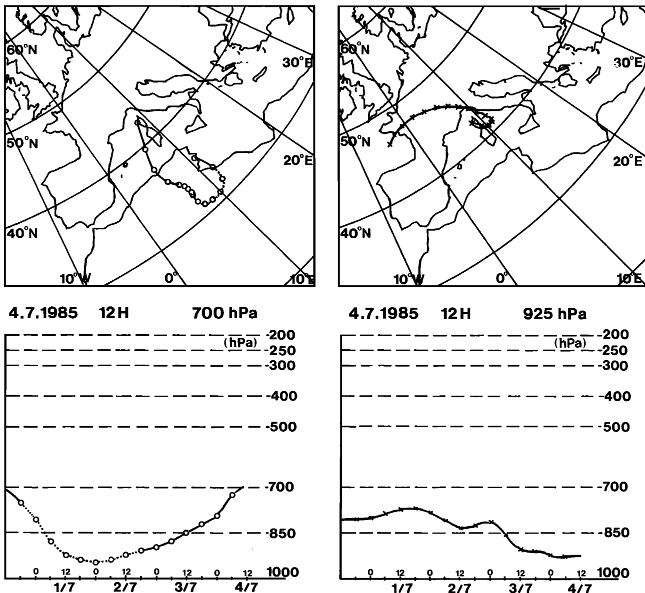
Fig. 2. Computed backward, three-dimensional air mass trajectories, ending at Capo Cavallo, at 1200 UT on July 4, 1985, at 700 and 925 hPa. The time step between consecutive marks is 6 hours.
