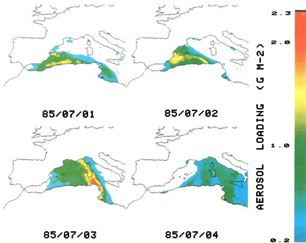
Plate 4. Computed desert aerosol columnar density ( \text{g m}^{-2} ) over the western Mediterranean at 1145 UT from July 1 to 4, 1985.
