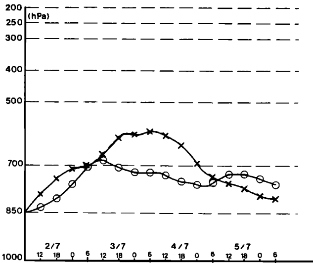
Fig. 3. Computed forward, three-dimensional air mass trajectories, leaving the eastern (o) and western (+) boundaries of the dust source area at 0600 UT on July 2, 1985, and at the 850 hPa initial level. The time step between consecutive marks is 6 hours.
