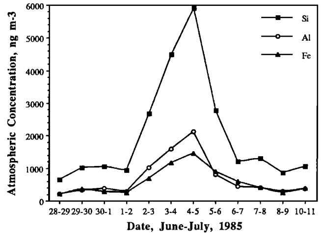
Fig. 4. Daily (noon to noon) mean atmospheric particulate concentrations of Si, Al, and Fe at Capo Cavallo between June 28-29 and July 10-11, 1985. The July 9-10 sample is missing.
