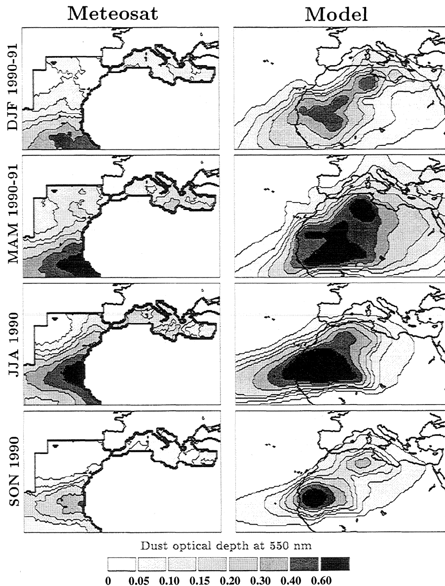
Figure 2. Seasonally averaged dust optical depths at 550 nm measured with Meteosat (left column) and simulated by the model (right column) for the pre-Pinatubo period January 1990 - June 1991. DJF: December, January, February. MAM: March, April, May. JJA: June, July, August. SON: September, October, November.
