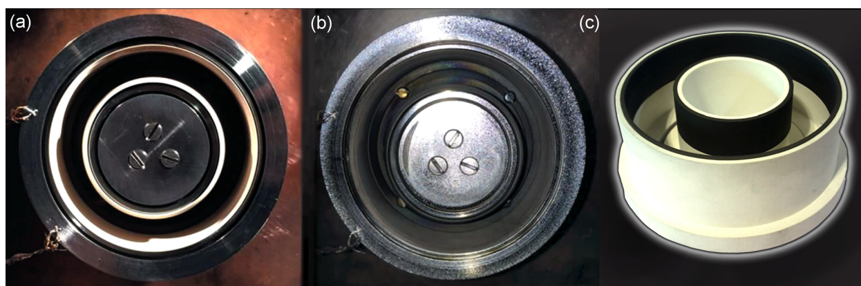
FIG. 10. A comparison of the MaSMi-60's discharge channel and pole faces before (a) and after ~20h of operation (b). Note the uniform layer of carbon deposited on the inner and outer channel walls, suggesting the presence of magnetic shielding, and the level of front inner and outer pole face erosion. Reprinted with permission from Conversano et al. , Paper IEPC-2015-100. Copyright 2015 EPRS. 63 (c) Conducting discharge channel walls with the graphite inserts for testing the magnetic shielding operational regimes. Reprinted with permission from J. Appl. Phys. 122, 033305 (2017). Copyright 2017 AIP Publishing LLC. 70
