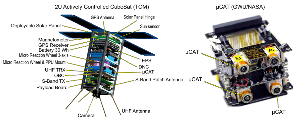
FIG. 26. (a) 2U Actively Controlled CubeSat (TOM) with \mu\text{CAT} thrusters installed and (b) NASA delivered hardware— \mu\text{CAT} (George Washington University/NASA). Courtesy: NASA. 196
