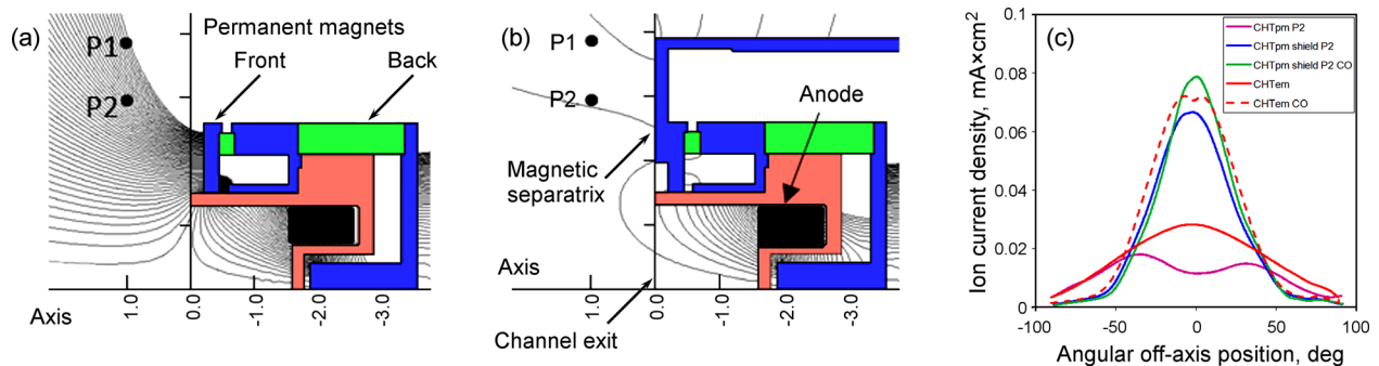
FIG. 7. A 2.6 cm diameter CHT with permanent magnets: (a) without the magnetic shield, B_{zmax} \approx 2.5 kGauss at the magnetic mirror and (b) with the magnetic shield, B_{zmax} \approx 1.8 kGauss. Magnetic iron parts made from a low carbon steel are marked in blue. Samarium-cobalt permanent magnets are marked in green. Two cathode placements, P1 and P2 used in CHTpm experiments are also shown. Reprinted with permission from J. Appl. Phys. 108 , 093307 (2010). Copyright 2010 AIP Publishing LLC. (c) Effect of the magnetic shield on the plasma plume of the CHTpm thruster. The results of the plume measurements for the CHTpm and CHTpm thrusters with the auxiliary keeper discharge [so-called current overrun (CO) regime] with the keeper current of 2.5 A] are also shown. All thrusters were operated at the discharge voltage of 250 V and Xenon gas flow rate of 0.35 mg/s. For the CHTpm thrusters, the cathode placement P2 is shown in (a) and (b). For the CHTpm thruster, the cathode outlet orifice was located approximately 5.4 cm away radially and 2 cm downstream from the center of the channel exit. All dimensions are in cm. Reprinted with permission from Raitseis et al. , Paper IEPC-2011-175. 46 Copyright 2011 ERPS.
