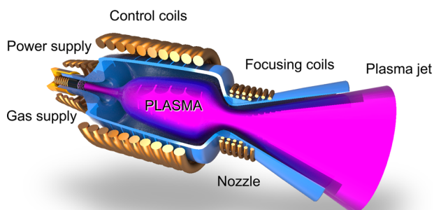
FIG. 19. Artistic representation of the Rotamak-based space propulsion thruster. Such a thruster could be capable of producing relatively high (reaching several N) thrust levels, provided the sufficient power supply levels.
