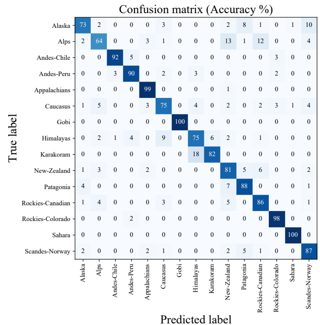
Fig. 8. Confusion matrix for 15 relief regions.
