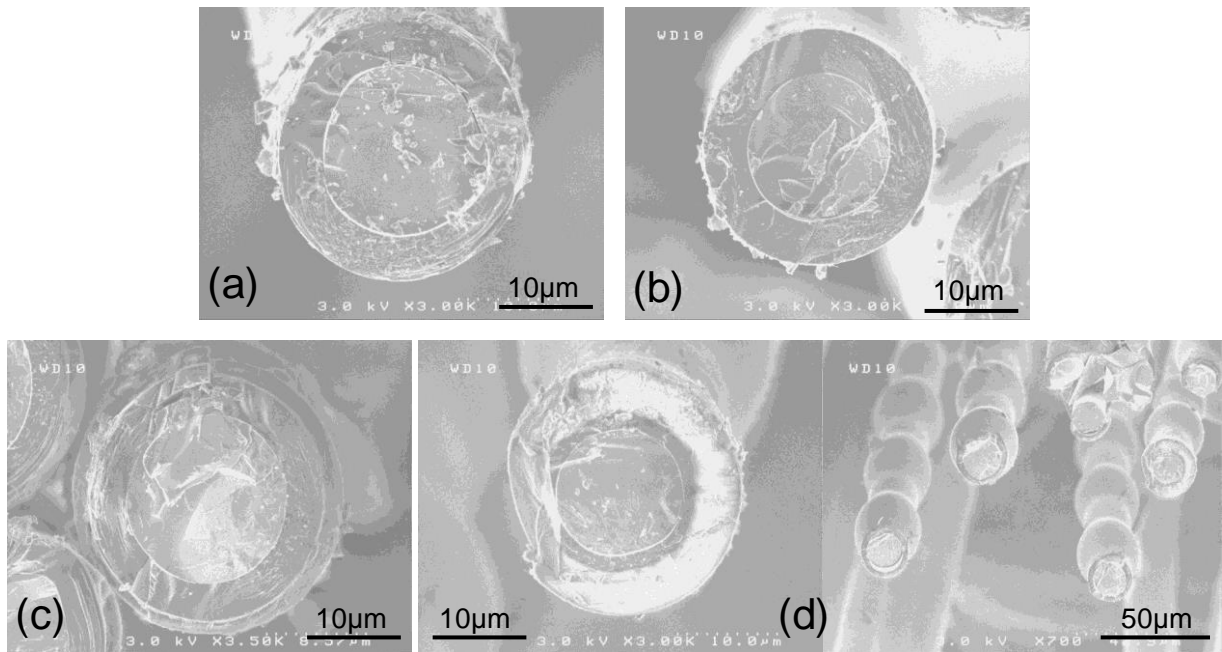
Figure 15: Cross section of S1 and S4 coatings on SiC fibers before: (a) S1, (b) S4, and after oxidation up to 700°C: (c) S1 and (d) S4.
