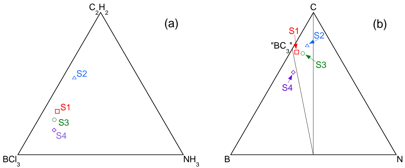
Figure 6: influence of the initial composition of the gas phase (a) on the atomic concentration of the \text{B}_x\text{C}_y\text{N}_z coatings (see Table 2), (b) ( P=4 kPa, T=1050^\circ\text{C} , Q_{\text{H}_2}=415 sccm)
