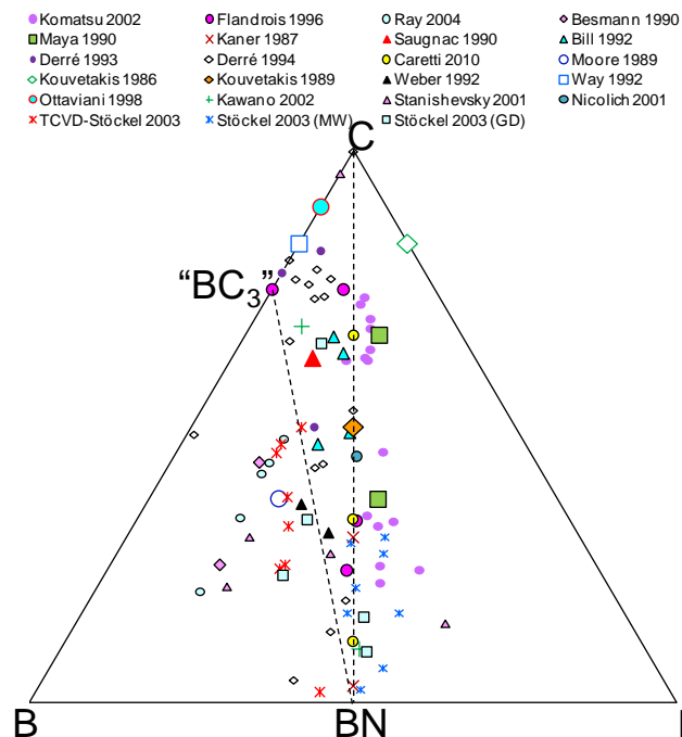
Figure 1: Examples of B_xC_yN_z coating compositions extracted from the literature
