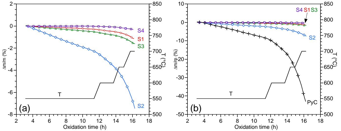
Figure 13: Weight change during the oxidation of \text{B}_x\text{C}_y\text{N}_z coatings in dry air between 550 and 700°C. (a) Comparison between S1 to S4. (b) Comparison between pyrocarbon and \text{B}_x\text{C}_y\text{N}_z coatings.
