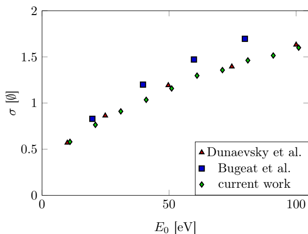
Fig. 4: Comparison between total electron emission yield of BN carried out in this study and extracted from literature.
