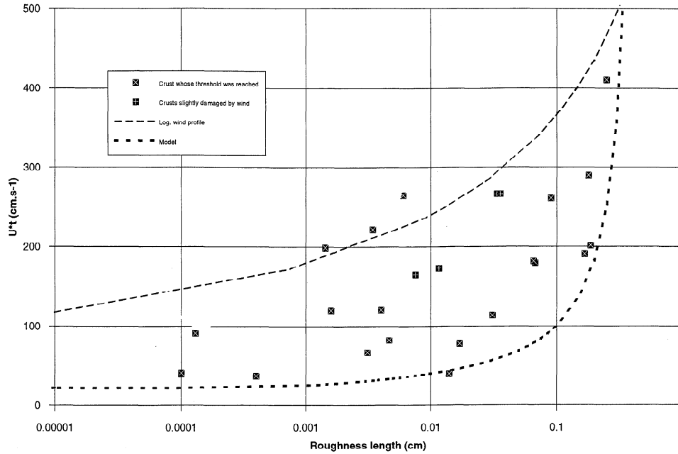
Figure 3. Values of u_{*t} versus z_0 for soils where the thresholds for crustal damage were reached. The long-dashed line shows the upper limit of u_{*t} , and the short-dashed line is the lowest limit for the exponential data simulated by the model (see Figure 3).
