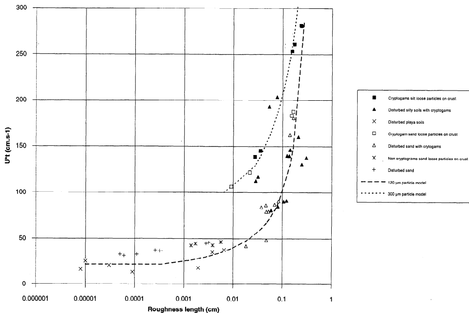
Figure 6. Observed u_{*c} for loose soils and for loose particles on cyanobacterial-lichen soil crusts. The long-dashed line is the model for loose soil u_{*c} ( 120 \mu\text{m} particles), and the short-dashed line is the model for 300 \mu\text{m} particles.
