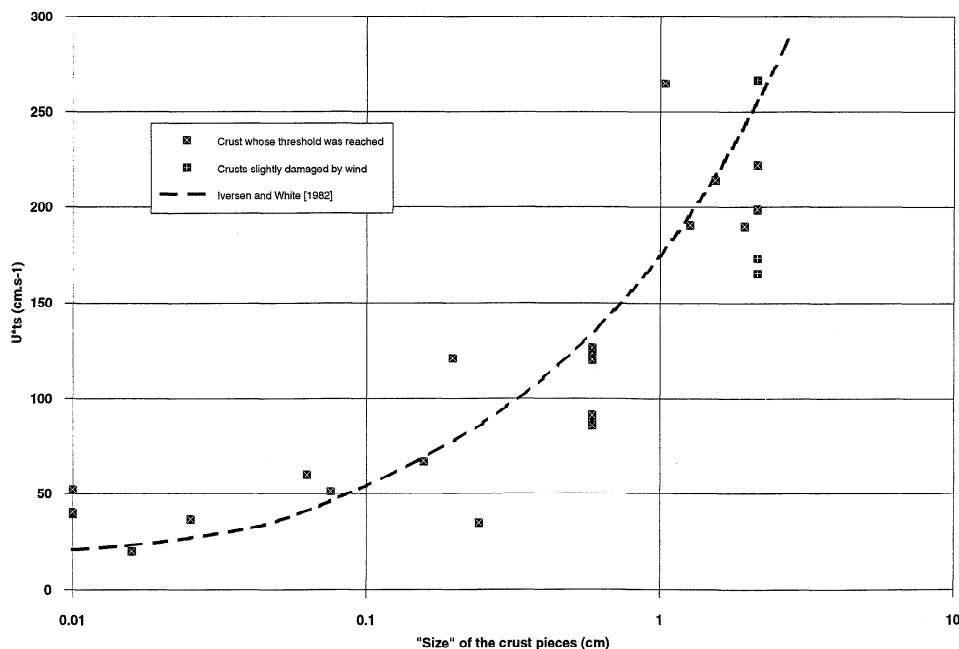
Figure 4. Observed u_{*ts} ( u_{*t} times f_{eff} , equivalent to the threshold friction velocity of the crust pieces) versus the equivalent size of a typical crust piece. Also shown is the theoretical curve of u_{*ts} = f(D_p) , derived by Iversen and White [1982].
