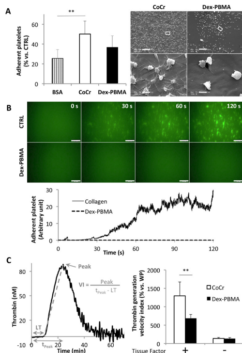
Fig. 3. Human platelet adhesion and thrombin generation on Dex-PBMA. (A) Left panel: Platelet adhesion in static condition on Dex-PBMA or CoCr discs and bovine serum albumin (BSA, negative control). Quantification of adherent platelets after 2h incubation at room temperature. Data are expressed as a percentage of adherent platelets on collagen (positive control). Values are mean \pm SEM of three determinations. **P < 0.01 . Right panel: Environmental scanning electron micrographs of adherent platelets on Dex-PBMA and CoCr. Scale bar 20 \mu m, higher magnification scale bar 2 \mu m. (B) Up: Dynamic adhesion of dioc-6 labeled platelets on Dex-PBMA and collagen coated glass-coverslips submitted to physiological flow (shear rate 1500 s^{-1} ). Micrographs of adherent platelets after 0, 30, 60 and 120 s. Down: Quantification of the adhesion within times on Dex-PBMA and collagen. (C) Thrombin generation on Dex-PBMA and CoCr discs. Left panel: Representative curve obtained after a thrombin generation experiment. Parameters of thrombin generation are shown: Lagtime (LT in min), time to peak ( t_{Peak} in min) and Peak (nM). Right panel: Velocity Indexes ( VI = \text{Peak} / (t_{Peak} - LT) ) for thrombin generation in PPP in the absence or presence of TF (1 \mu M) on Dex-PBMA and CoCr. Data are expressed as a percentage of the results on well plate (WP). Values are mean \pm SEM of six determinations. **P < 0.01 .
