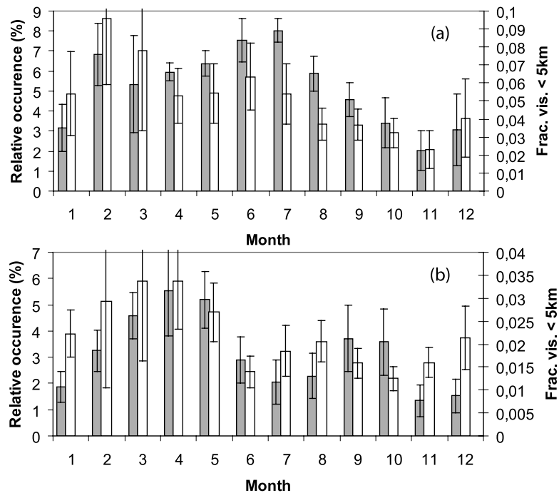
Figure 8. Average monthly relative occurrence of dust emissions (1996–2001, simulated with 6-h step) in % (in grey), and the fraction of observations with visibility less than 5 km (in white) [Mahowald et al. , 2007], for the (a) western Sahara and (b) eastern Sahara. The error bars indicate the standard deviation associated to the mean value.
