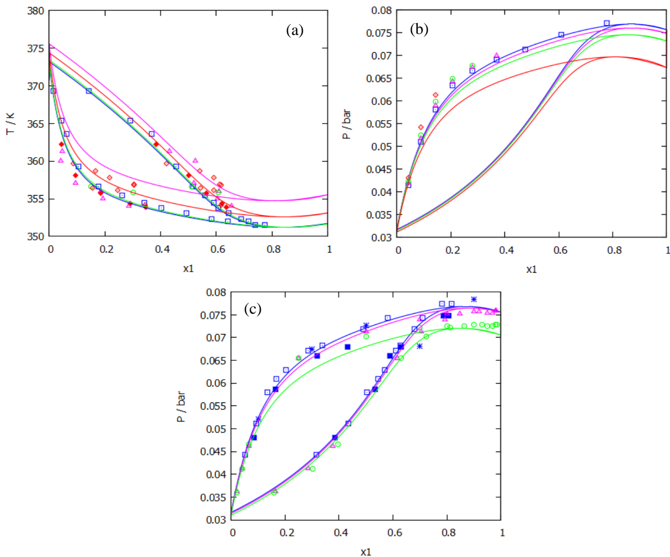
Fig. 9. VLE of ethanol (1) -water (2) with: (a) NaCl at P=1.01\text{bar} for x_{\text{NaCl}}=0 ( \square ), x_{\text{NaCl}}=0.01 ( \odot ), x_{\text{NaCl}}=0.03 ( \diamond , \blacklozenge ), x_{\text{NaCl}}=0.05 ( \blacktriangle ), (b) KCl at T=298\text{K} for m_s=0 ( \square ), m_s=0.3 ( \blacktriangle ), m_s=0.5 ( \odot ), m_s=1 ( \blacklozenge ), (c) LiCl at T=298\text{K} for m_s=0 ( \square ), m_s=0.5 ( \blacktriangle ), m_s=1 ( \odot ). Calculation with the NRTL-PRA EoS (—).
