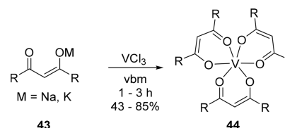
Scheme 10. Mechanochemical Synthesis of Vanadium(III) \beta -Diketonates
