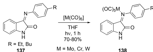
Scheme 32. Photosynthesis of [M(CO)_5(L)] Complexes
