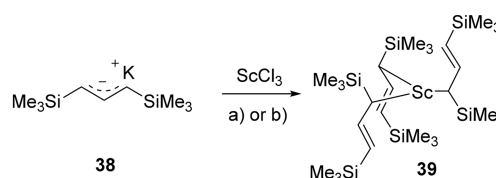
Scheme 8. Mechanochemical Synthesis of Tris(allyl)scandium Species 39
