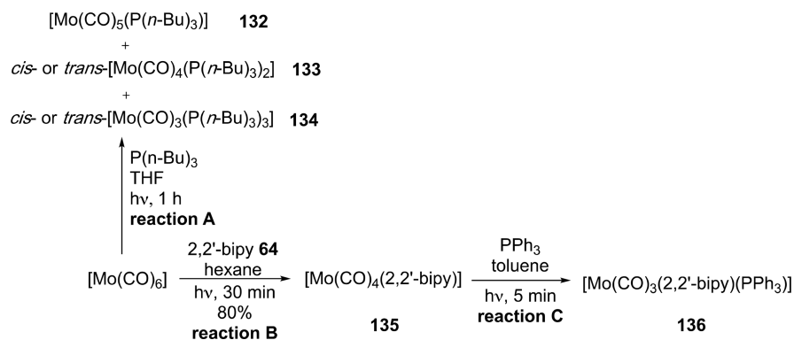
Scheme 31. Photochemical Reaction of [Mo(CO)_6]
