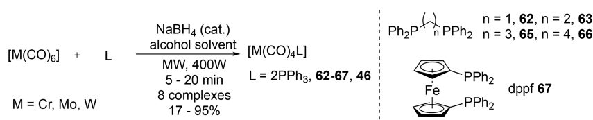
Scheme 18. Microwave-Assisted Synthesis of Group 6 Complexes Using NaBH 4 as Catalyst
