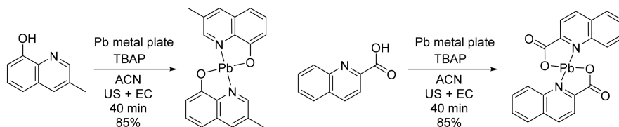
Scheme 188. Sonochemical Synthesis of Lead(II) Complexes of O-,N-Coordinating Ligand
