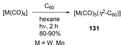
Scheme 30. Photochemical Synthesis of [M(CO)_5(\eta^2-C_{60})]
