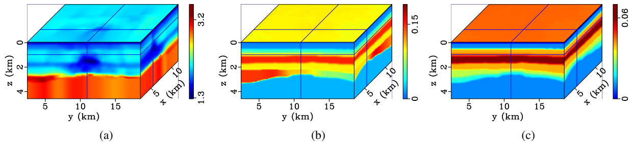
Figure 1: Initial (a) P-wave vertical velocity V_{P0} , and the anisotropy coefficients (b) \epsilon and (c) \delta .
