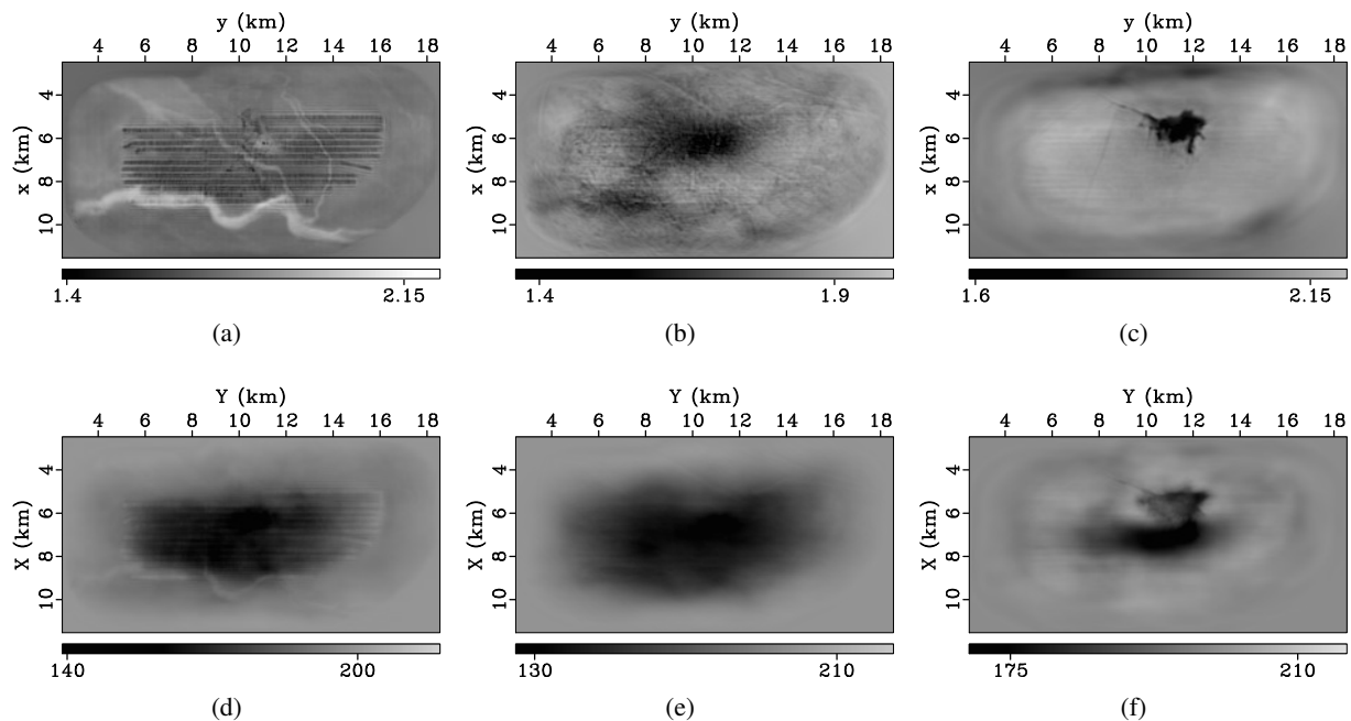
Figure 4: Velocities at (a) z = 200 m, (b) z = 500 m, and (c) z = 1000 m obtained from joint inversion of V_{P0} and Q_p using depth-preconditioning, for frequencies in the data up to 7 Hz. The inverted attenuation Q_p at depths of (d) 200 m, (e) 500 m, and (f) 1000 m.
