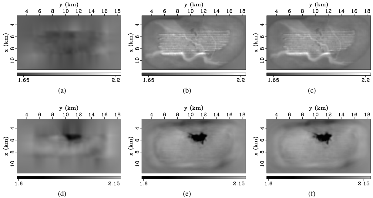
Figure 2: (a) Initial P-wave vertical velocity V_{P0} at a depth of 200 m. The V_{P0} at the same depth obtained after FWI (b) without attenuation, and (c) in viscous media. The (d) initial V_{P0} at a depth of 1000 m, inversion results (e) in the absence and (f) in the presence of attenuation. The units of velocity here, and in the following figures are km/s.
