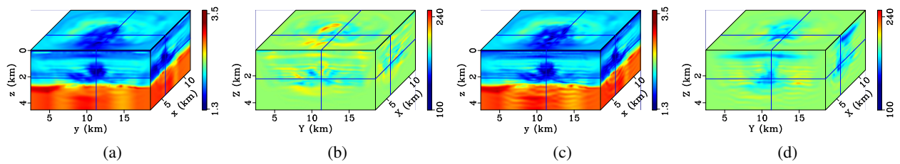
Figure 3: Joint inversion of velocity and attenuation: (a) P-wave vertical velocity V_{P0} and (b) attenuation Q_p obtained using pseudo-Hessian preconditioner. The inverted (c) V_{P0} and (d) Q_p from depth-preconditioning.
