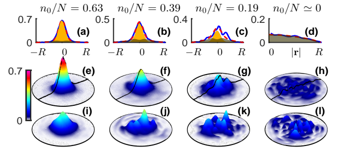
FIG. 3: Experiments. Intensity patterns recorded at Z_0 = 20\text{cm} (bottom line), and at the output of the whole fiber length L = 13\text{m} (middle line): By reducing the number of modes initially excited (i.e., by decreasing E ), a transition occurs from n_0 = 0 to a condensate fraction of n_0/N \simeq 0.63 . (a-d) The fundamental Gaussian mode u_0(\mathbf{r}) of the MMF gets macroscopically populated as evidenced by the intensity line-outs I(x, y = 0) recorded experimentally at z = L (blue line), and the corresponding fits of the condensate contribution I_{\text{cond}}(\mathbf{r}) (orange filled region), and of the incoherent contribution I_{\text{inc}}(\mathbf{r}) (grey filled region). The red-dashed line denotes I_{\text{cond}}(\mathbf{r}) + I_{\text{inc}}(\mathbf{r}) . Above the transition to condensation n_0 = 0 (d), we computed the angle averaged distance |\mathbf{r}| of the intensity recorded experimentally (blue), which is in agreement with the Rayleigh-Jeans distribution I_{\text{inc}}(\mathbf{r}) (red-dashed). R = 26\mu\text{m} is the fiber core radius (corresponding to the circles (e-l)), N_* = 120 modes, N = 19\text{kW} .
