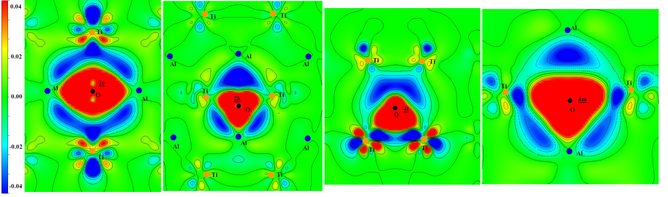
Figure 4. Charge transfer, \Delta\rho (in e/\text{\AA}^3 ), when sites are filled: oxygen in 2e (2D data displays in the [10\text{-}1] direction), 2h ( [-110] ), 4i ( [-100] ) and 4m ( [1\text{-}10] ) sites. Al atoms are in blue, Ti atoms in orange and O in black.
