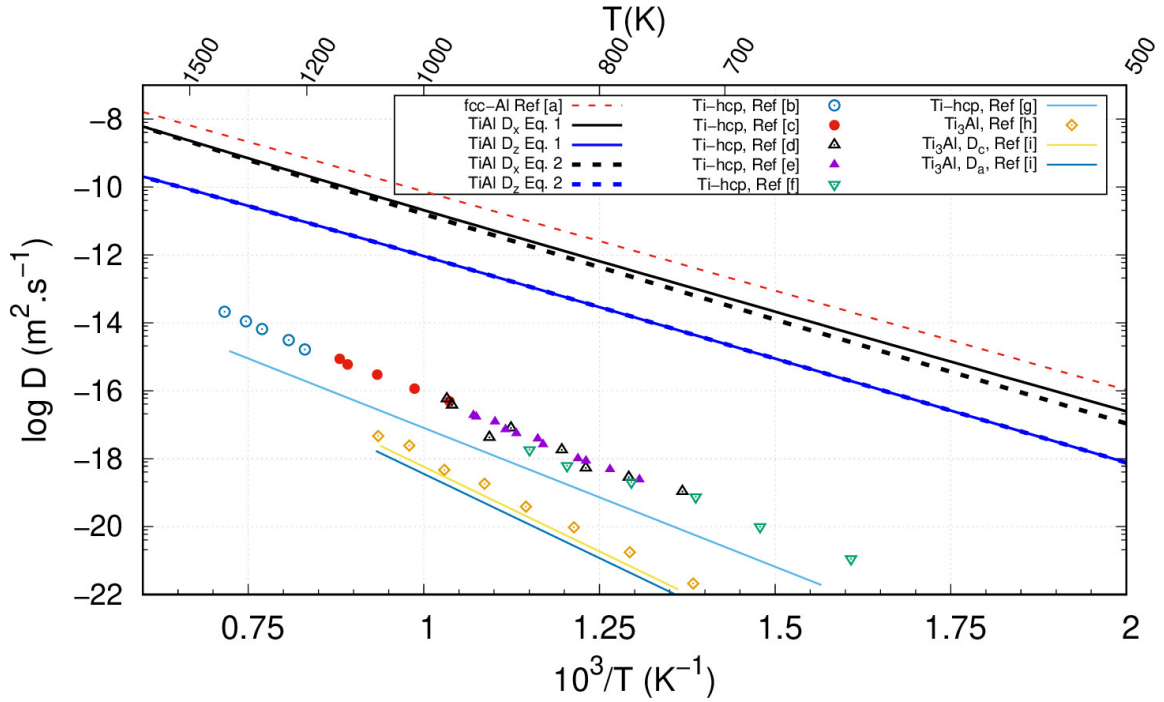
Figure 6. Diffusion coefficients of oxygen as a function of 1/T . Al Ref.: [a]=[28]; Ti-hcp Ref.: [b]=[29], [c]=[30],; [d]=[31], [e]=[32], [f]=[33], [g]=[34]; Ti 3 Al Ref.: [h]=[35]; [i]=[24].
