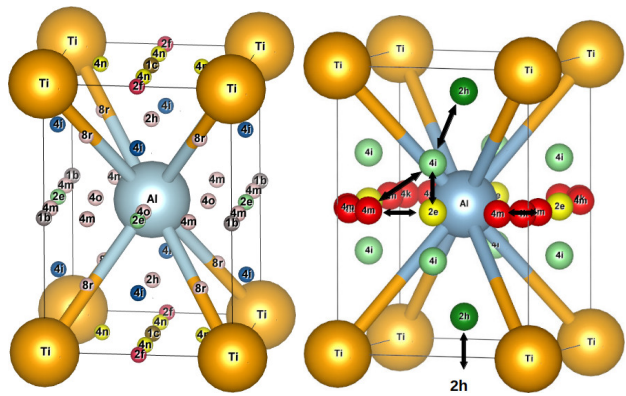
Figure 1. Schematic representations of the TiAl- L1_0 structure (bold-centered tetragonal representation) indicating the interstitial positions tested (left), and the stable positions (right).
