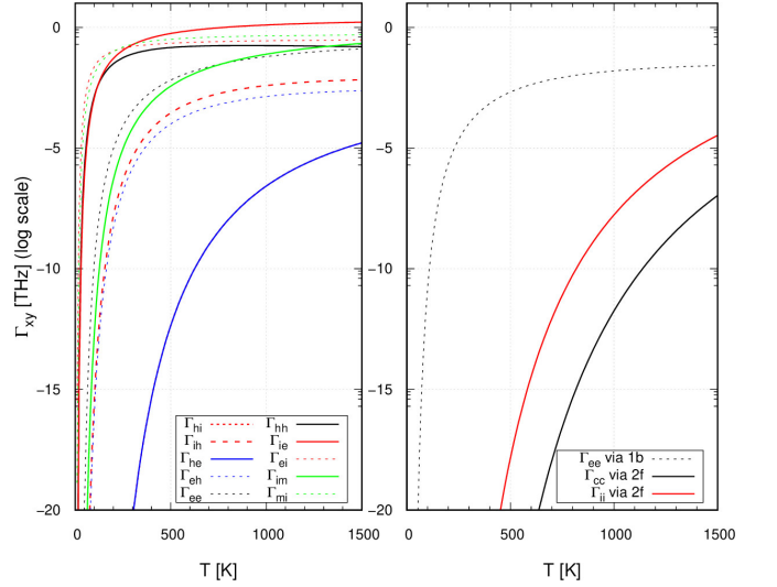
Figure 7. Attempt frequencies of all jumps as a function of T .
