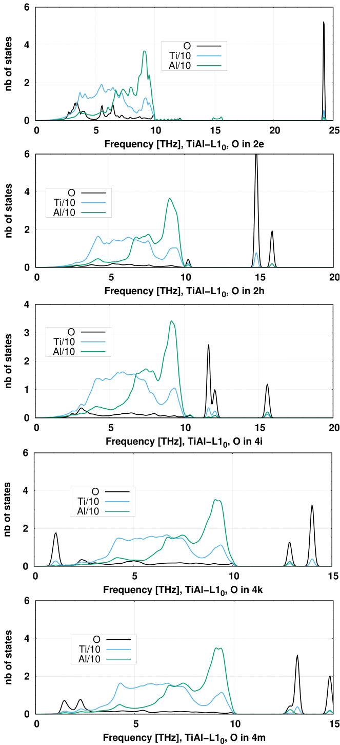
Figure 3. From top to bottom, pDOS of O in the 2e , 2h , 4i , 4k or 4m sites.
