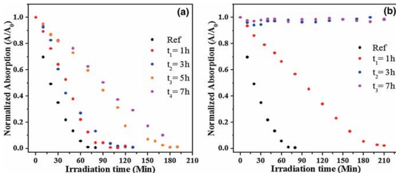
Figure 8. Photo-catalytic degradation, over time, of methylen orange in aqueous solution in the presence of TiO 2 NPs, for the milling times: t = 0 (reference), 1, 3, 5, 7 h at \Omega = (a) 200 and (b) 400 rpm.
