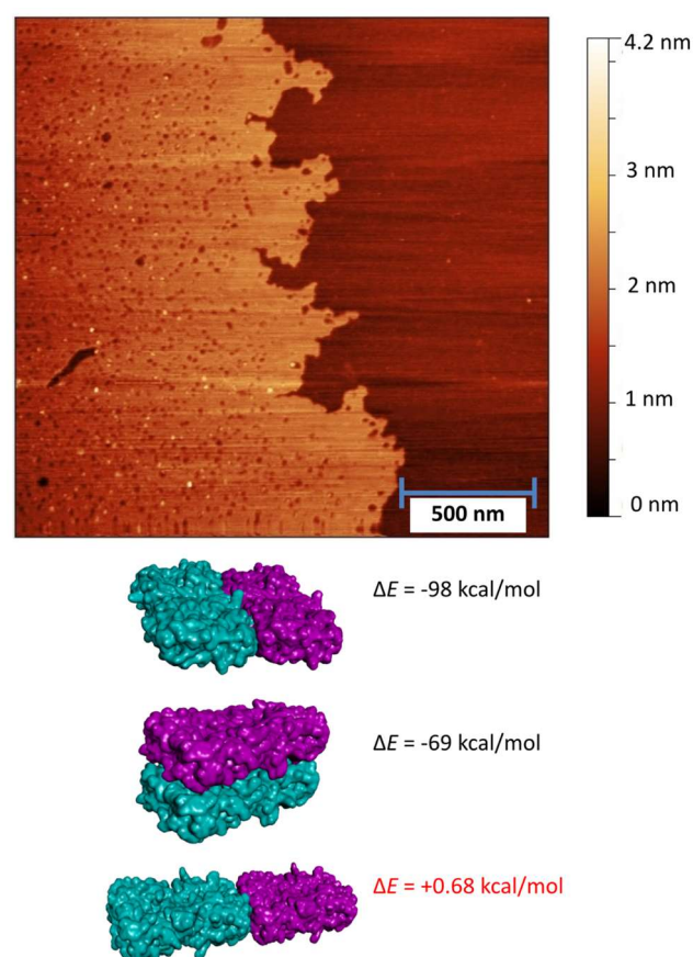
Figure 4: AFM topographic image of M4-LecA complex, image size 2 \times 2 \mu\text{m}^2 and MD simulation of lectin/lectin interaction.
