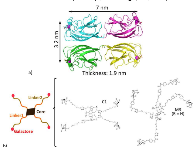
Figure 1: (a) Crystal structure of LecA complex with GalA-QRS at 2.31 Å resolution (RCSB code 4LKD, https://www.rcsb.org/structure/4LKD ); (b) Schematic of the general structure of the glycoclusters and two examples of the glycoclusters studied, namely C1 and M3. All the structures are given in the Supporting Information.
