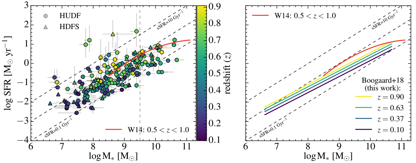
Fig. 7. Left panel: sample of 179 star-forming galaxies observed with MUSE, plotted on the M_* -SFR plane. The symbols indicate the field and colour indicates the redshift. The dashed lines show a constant sSFR, which is equivalent to a linear relationship: \text{SFR} \propto M_* . The red curve shows the model of the star formation sequence from Whitaker et al. (2014) for 0.5 < z < 1.0 . The vertical grey dashed line indicates the selection for the low-mass fit (Sect. 5.2). Right panel: same as the left panel but with the data points removed, showing (the evolution of) the star formation sequence as seen by MUSE, according to Eq. (11).
