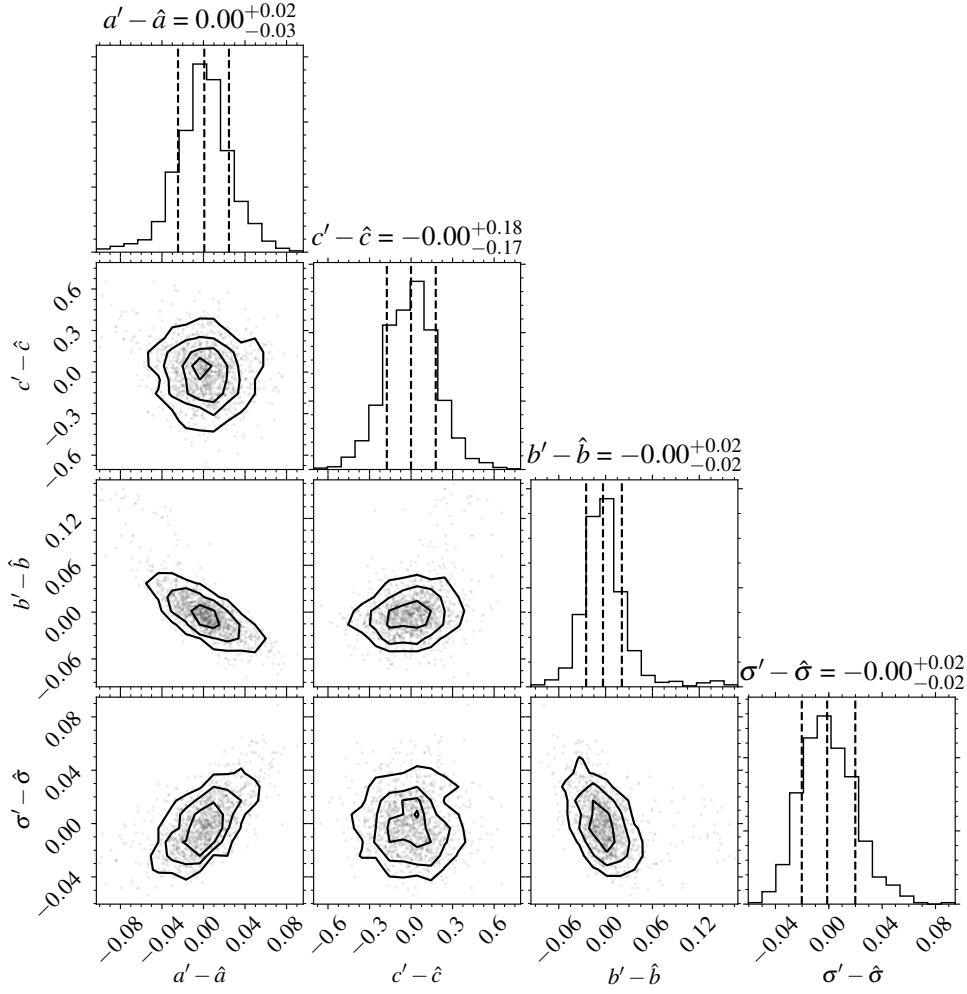
Fig. A.2. Differences between the recovered parameters, \mathbf{x}'_{\text{true}} = (a', c', b', \sigma'_{\text{intr}})^T and the true parameters, \mathbf{x}_{\text{true}} = (\hat{a}, \hat{c}, \hat{b}, \hat{\sigma}_{\text{intr}})^T , for the N = 1260 points from our simulation; see Eq. (A.3). We can recover the input parameters of our simulation very well, with no mean offset and very small scatter (compared to the uncertainty on each parameter obtained from the observations). Figure created using the corner.py module (Foreman-Mackey 2016).
