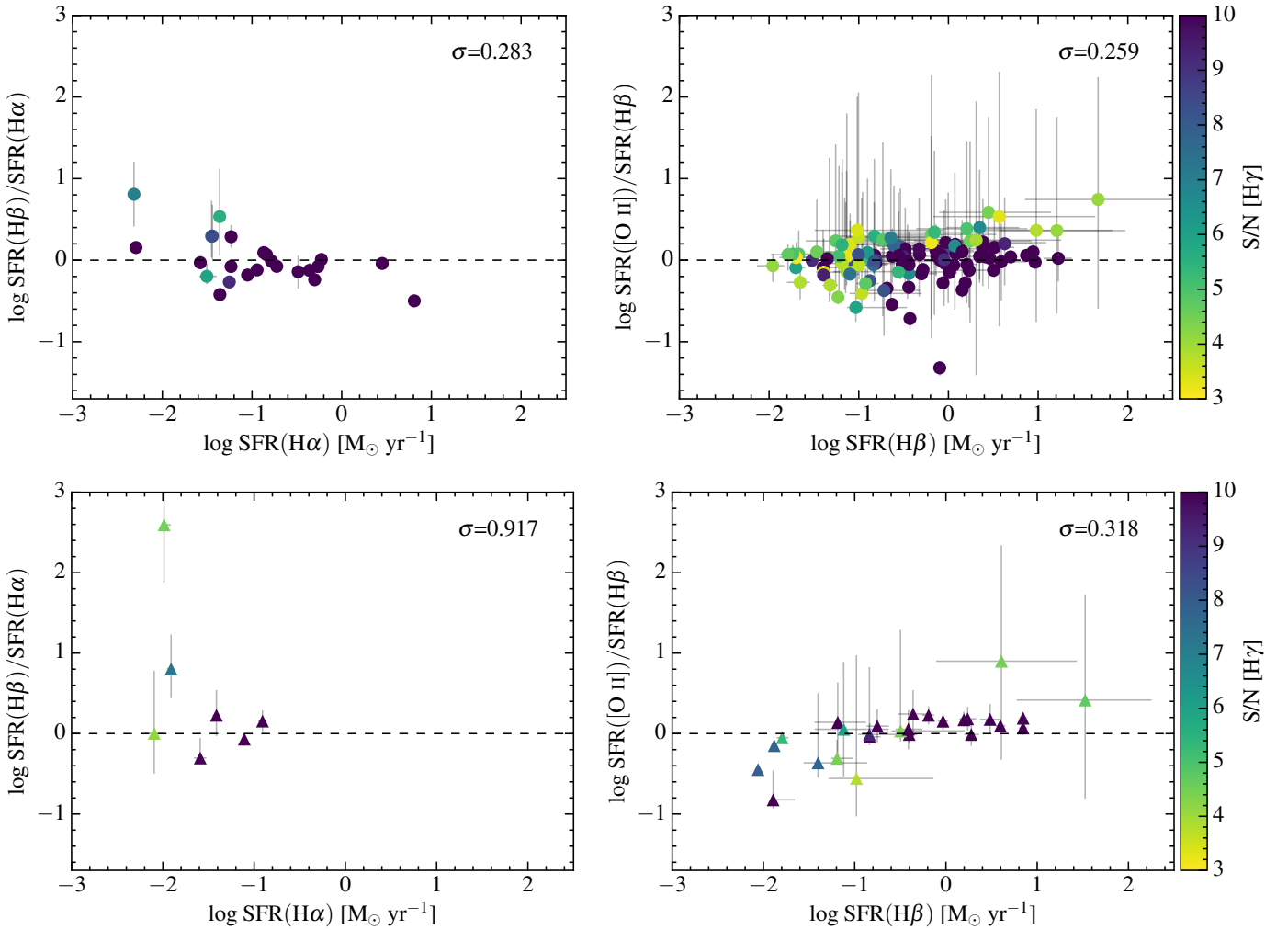
Fig. 5. A comparison of the derived star formation rate (SFR) from the H\alpha \lambda 6563 , H\beta \lambda 4861 and [O II] \lambda 3727 luminosities for the HUDF ( top panels , circles) and the HDF5 ( bottom panels , triangles). Left panels : logarithm of the SFR from H\alpha \lambda 6563 vs. the difference between the log H\beta \lambda 4861 and log H\alpha \lambda 6563 SFRs. Right panels : same for H\beta \lambda 4861 vs. [O II] \lambda 3727 . In each panel \sigma indicates the standard deviation (in dex) around the one-to-one relation. Colour indicates the signal-to-noise ratio (S/N) in the faintest line; H\gamma \lambda 4340 . Only galaxies that allowed for more than one SFR indicator are included in the plot. Overall the SFRs from H\beta \lambda 4861 and [O II] \lambda 3727 agree reasonably well, considering we have not taken into account the metallicity dependence in SFR([O II] \lambda 3727) . The scatter in H\alpha \lambda 6563 vs. H\beta \lambda 4861 SFR is largely driven by H\gamma \lambda 4340 S/N.
