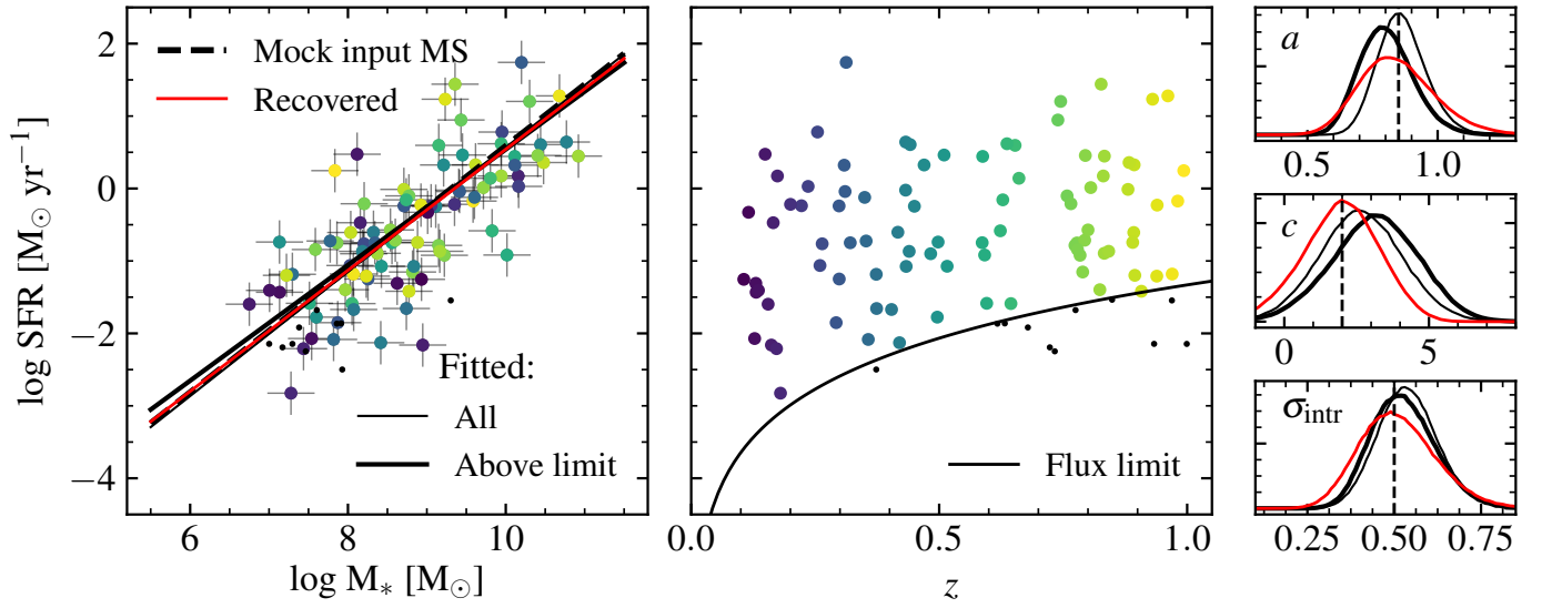
Fig. A.1. Results from the recovery experiment on mock galaxies. The points in the left and centre panels show one of the 30 realisations of 100 galaxies in (\log M_*, \log(1+z), \log \text{SFR}) -space from a mock star formation sequence: \log \text{SFR} \propto a \log M_* + c \log(1+z) , where in this particular case a = 0.8 and c = 2.0 with \sigma_{\text{intr}} = 0.5 dex. The colour indicates redshift, unless a mock galaxy falls below the solid line in the centre panel, indicating the flux limit of \sim 3 \times 10^{-19} \text{ erg s}^{-1} \text{ cm}^{-2} , in which case it is a black point. The rightmost panels show the marginalised distributions (slope, redshift evolution, and intrinsic scatter) from combining all 30 realisations for this particular set of parameters. The thin and thick black lines indicate the results when taking into account all mock data and only the data above the flux limit, respectively, and are compared to the input values (dashed lines). With all data points (including noise), we can recover the input parameters sequence well. When applying the flux limit a slight bias towards a shallower slope and steeper redshift evolution appears. We plot all curves in the leftmost panel at the average redshift of the sample ( z_0 ). The red line is obtained after applying the correction to the fit of the data above the limit. These recovered curves are plotted in the leftmost panel as well and compared to the input mock relation. With our correction, we can recover the true input parameters well, even in the case of limited data.
