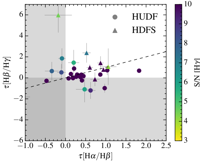
Fig. 6. Optical depths at the wavelength of H\beta \lambda 4861 as derived from both the H\beta \lambda 4861/H\gamma \lambda 4340 and the H\alpha \lambda 6563/H\beta \lambda 4861 -ratio, coloured by H\gamma \lambda 4340 signal-to-noise (S/N). The dashed line is the one-to-one relation. Overall the optical depths agree reasonably well, unless the H\gamma S/N is low. Most galaxies actually show little dust ( \tau close to zero). The shaded area shows the regions of (unphysical) negative optical depth for each axis. We set the optical depth to zero for galaxies with negative \tau as this is often consistent with the error bars and the offset is due to noise in the spectra. We note that some of the high-S/N outliers actually have discrepant Balmer ratios. If the inferred optical depth is very different, this will affect the comparison of the dust-corrected SFR from H\beta \lambda 4861 and H\alpha \lambda 6563 (see Fig. 5).
