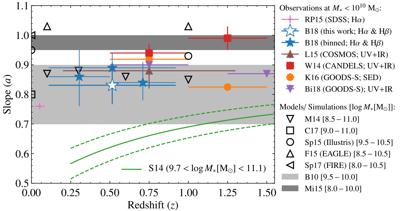
Fig. 10. A comparison of the slope ( a ) as a function of redshift ( z ) with studies from the literature that extend down to M_* < 10^{10} M_\odot near our redshift range. Our best-fit (bias-corrected) slope from Eq. (11) is shown by the large star. As most studies have probed the slope in bins of redshift, we also include our results obtained using non-evolving redshift bins (Eqs. (14), (15) and (16); smaller blue stars). The literature results are from Renzi & Peng (2015, RP15) , Kurczynski et al. (2016, K16) , Bisigello et al. (2018, B18) and the low-mass ( M_* \lesssim 10^{10} M_\odot ) power-law slopes from Whitaker et al. (2014, W14) and Lee et al. (2015, L15) . We also add Speagle et al. (2014, SP14) for reference, though it is inferred at higher masses. We indicate the field and SFR-tracer in brackets, though note that distinct calibrations for the same tracer may be used in different studies. In addition, we add the slopes predicted by (semi-)analytical models; Bouché et al. (2010, B10) , Mitchell et al. (2014, M14) , Mitra et al. (2015, Mi15) , Cattaneo et al. (2017, C17) , and hydrodynamical simulations; Sparre et al. (2015, Sp15) , Furlong et al. (2015, F15) , Sparre et al. (2017, Sp17) .
