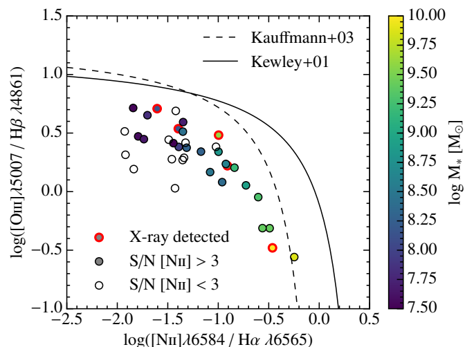
Fig. 2. BPT-diagram (Baldwin et al. 1981) of the sources in our H\alpha \lambda 6563 -subsample for which we measure [\text{N II}] \lambda 6584 . All galaxies fall in the star-forming region of the diagram. The filled and open circles have S/N([\text{N II}] \lambda 6584) > 3 and < 3 , respectively, and the 5 sources encircled in red are detected in X-rays (Luo et al. 2016). The solid and dashed curve show the AGN boundary and maximum starburst line from Kauffmann et al. (2003) and Kewley et al. (2001), respectively.
