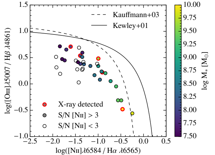
Fig. 2. BPT-diagram (Baldwin et al. 1981) of the sources in our H\alpha \lambda 6563 -subsample for which we measure [\text{N II}] \lambda 6584 . All galaxies fall in the star-forming region of the diagram. The filled and open circles have S/N([\text{N II}] \lambda 6584) > 3 and < 3 , respectively, and the 5 sources encircled in red are detected in X-rays (Luo et al. 2016). The solid and dashed curve show the AGN boundary and maximum starburst line from Kauffmann et al. (2003) and Kewley et al. (2001), respectively.
