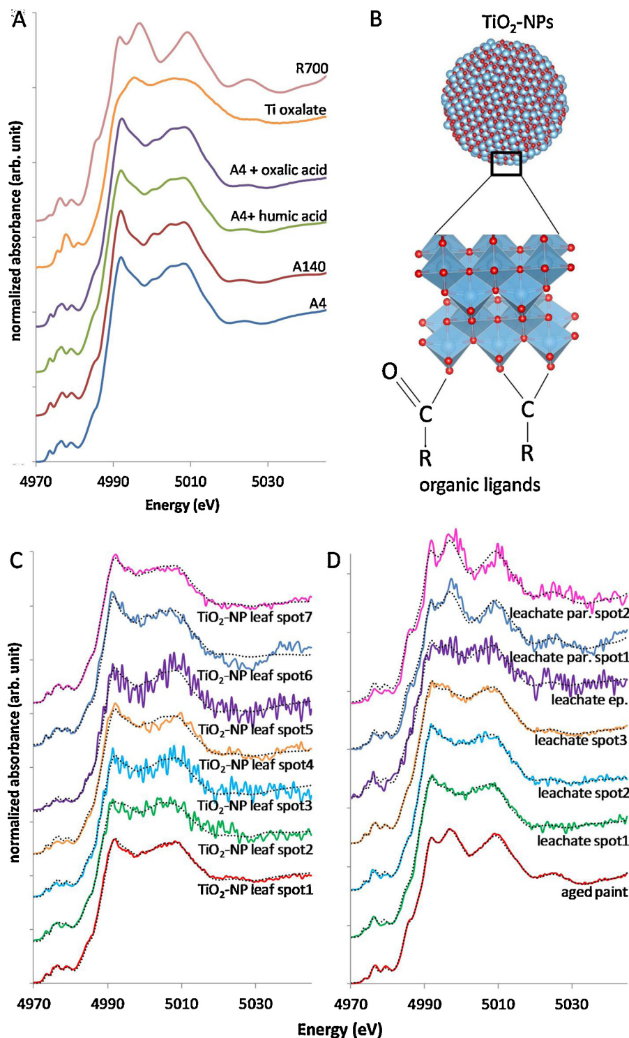
Fig. 4. (A) XANES spectra of the reference compounds; (B) possible interactions between nano anatase surface and organic ligands; \mu XANES spectra obtained in situ on lettuce leaves exposed to 1250 nmol g -1 TiO 2 -NPs (C) or to aged paint leachate (D). Dotted lines figure the best linear combination fits obtained with reference compounds (par., parenchyma; ep., epidermis; A., anatase; R., rutile).
