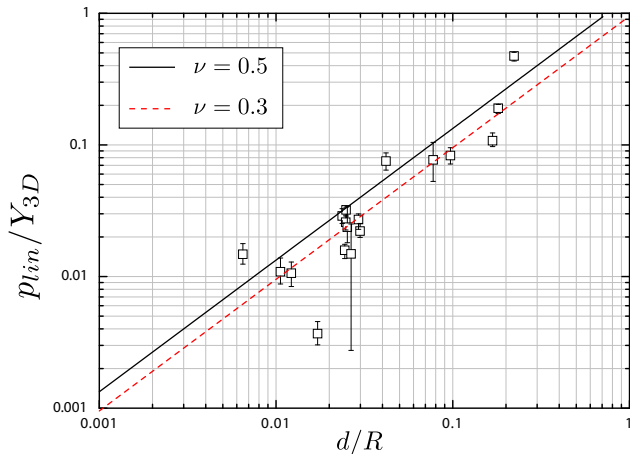
Fig. 12. Slope p_{lin} of the linear part of the \Delta P \left( \frac{\Delta V}{V_0} \right) diagram, adimensionnalized by the Young modulus Y_{3D} directly measured from traction experiments. Straight lines : theoretical curves for p_{lin}/Y_{3D} = \frac{2}{3(1-\nu)} \times \frac{d}{R} , displayed for two values typically bounding the Poisson's ratio of the shells studied.
