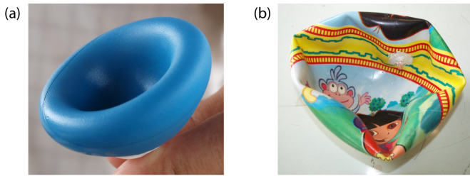
Fig. 2. Elastic shells almost fully deflated; the hemisphere that is curved inward is in contact with the, mainly unchanged, other half of the shell. (a) Thick shell (relative thickness d/R = 0.18 ; external radius R + d/2 = 55.5 mm), in which axisymmetry was conserved throughout the deflation. (b) Thin shell ( d/R = 10.6 \cdot 10^{-3} ; external radius R + d/2 = 190 mm), where radial folds began to develop inside the depression at some point of the deflation process.
